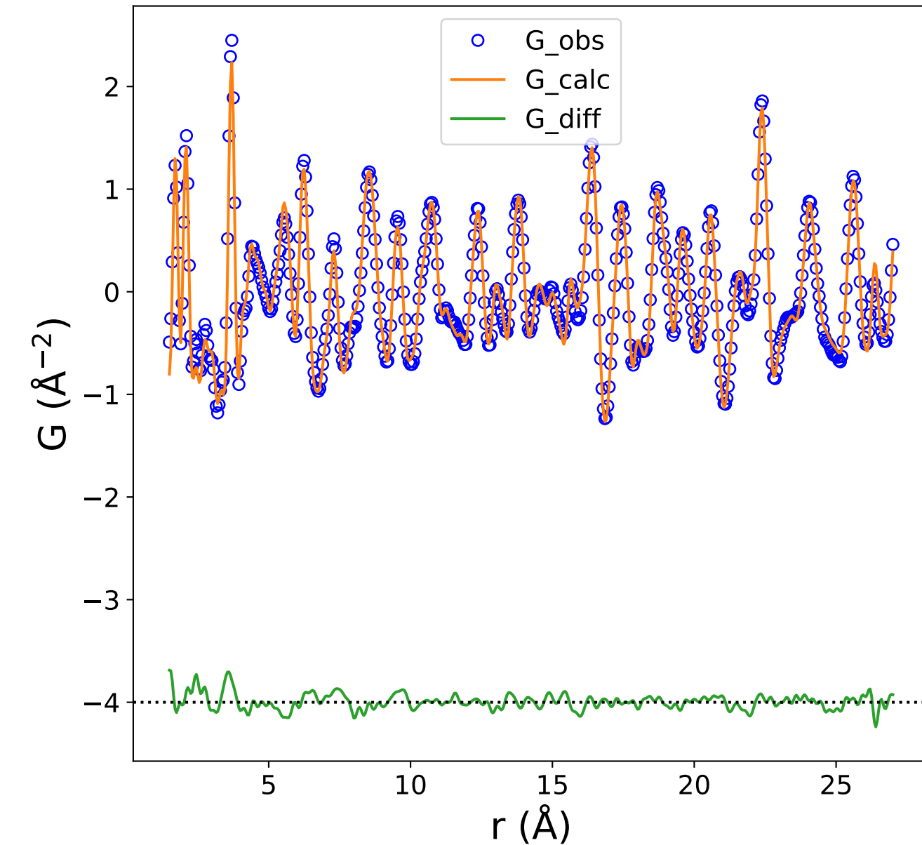
PDF Data and Fit (Rw = 0.126)
