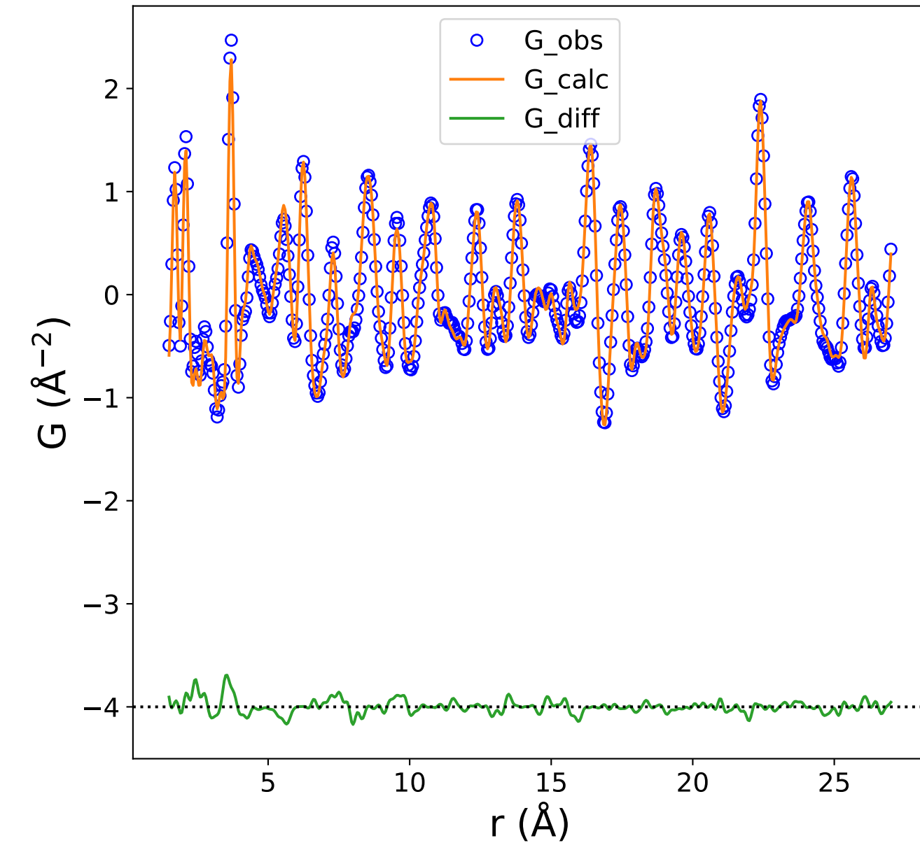
PDF Data and Fit (Rw = 0.109)
