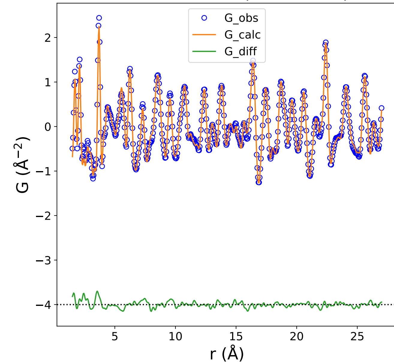
PDF Data and Fit (Rw = 0.116)
