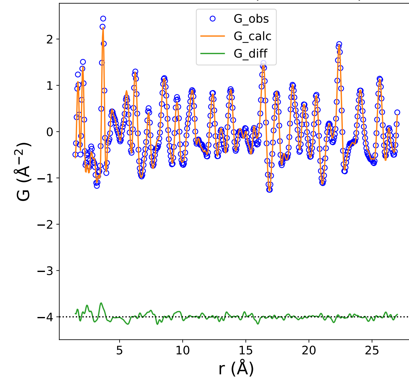
PDF Data and Fit (Rw = 0.110)
