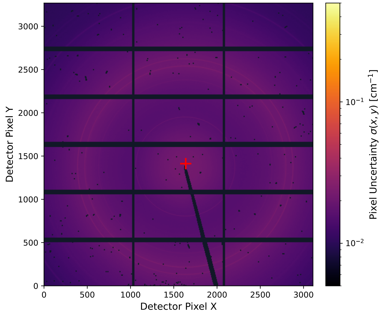
(a) Propagated 2D Uncertainty \sigma(x, y) [ \text{cm}^{-1} ]
