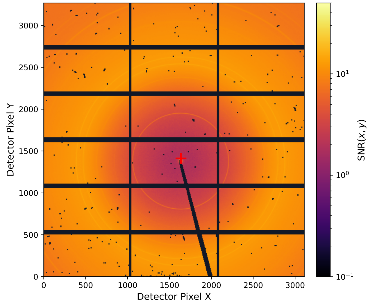
(b) Pixel Signal-to-Noise Ratio \text{SNR}(x, y) = |I_{\text{sub}}|/\sigma
