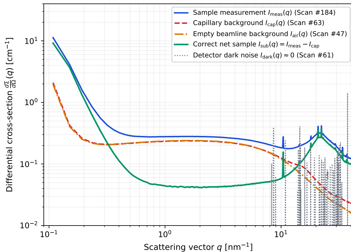
(a) Complete scattering decomposition across full q -range
