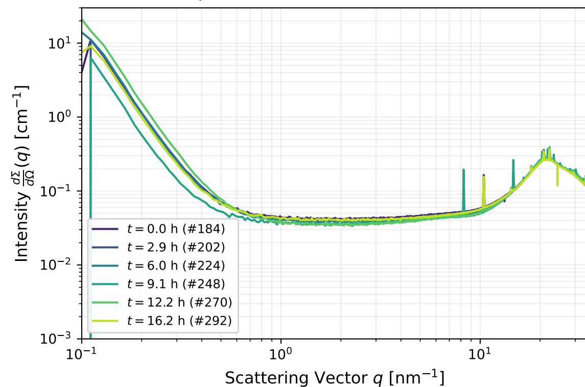
(c) Representative SAXS Curves Over Time
