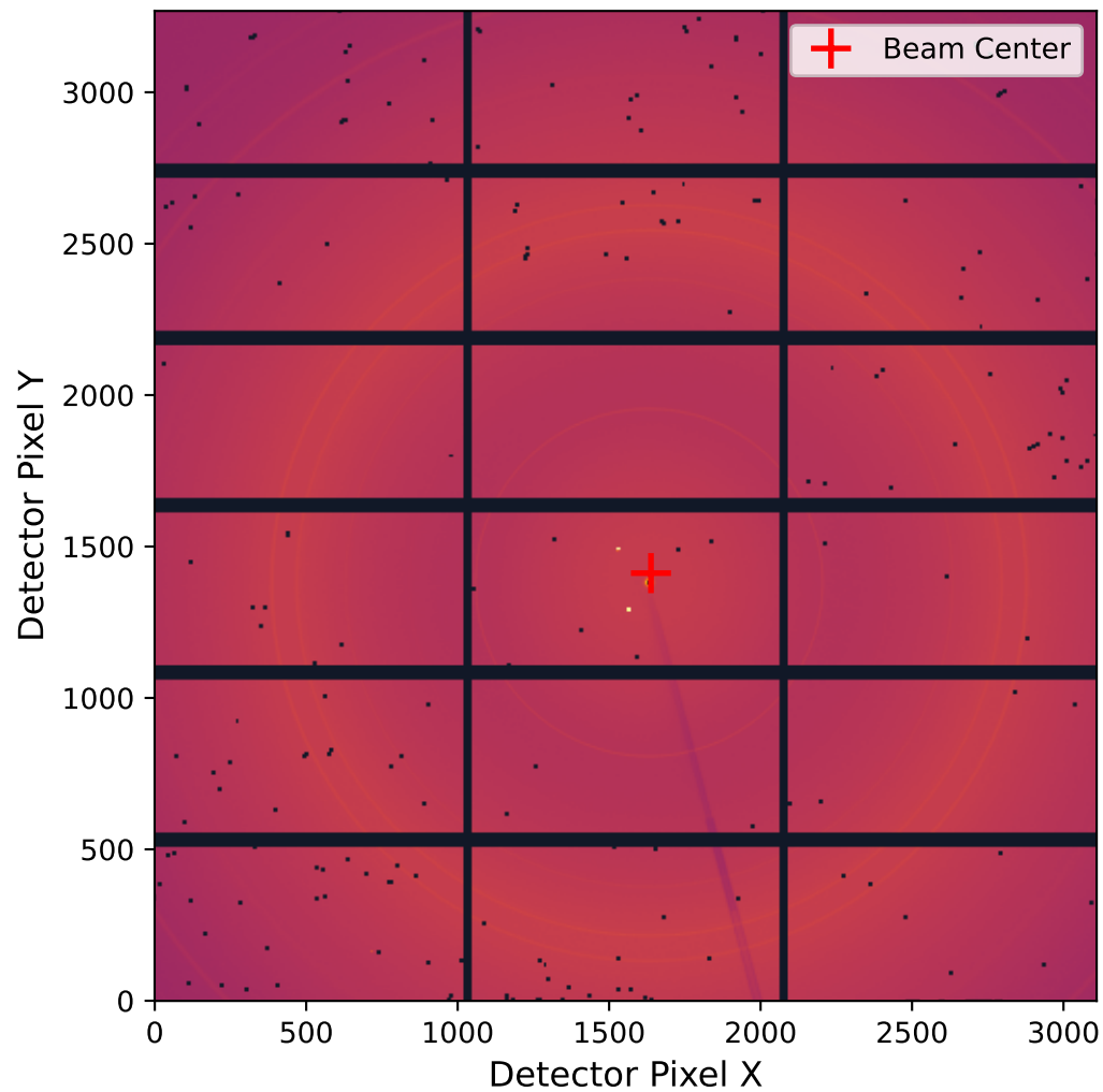
(a) Sample Raw 2D Frame (#184)
