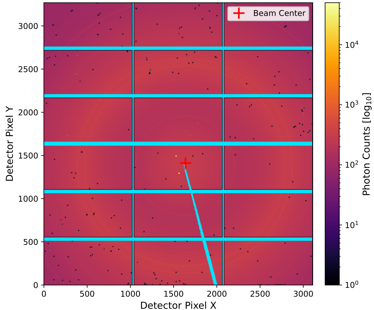
(b) Active Data Area (Mask Shaded in Cyan)
