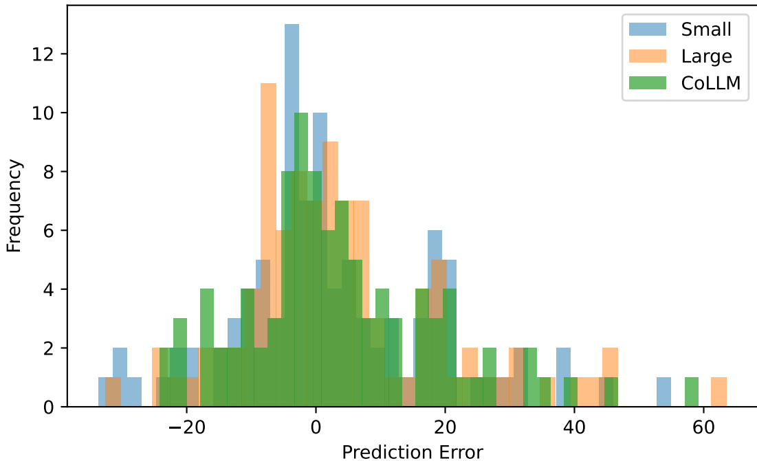
Error Distribution on Test Set (FD003)
