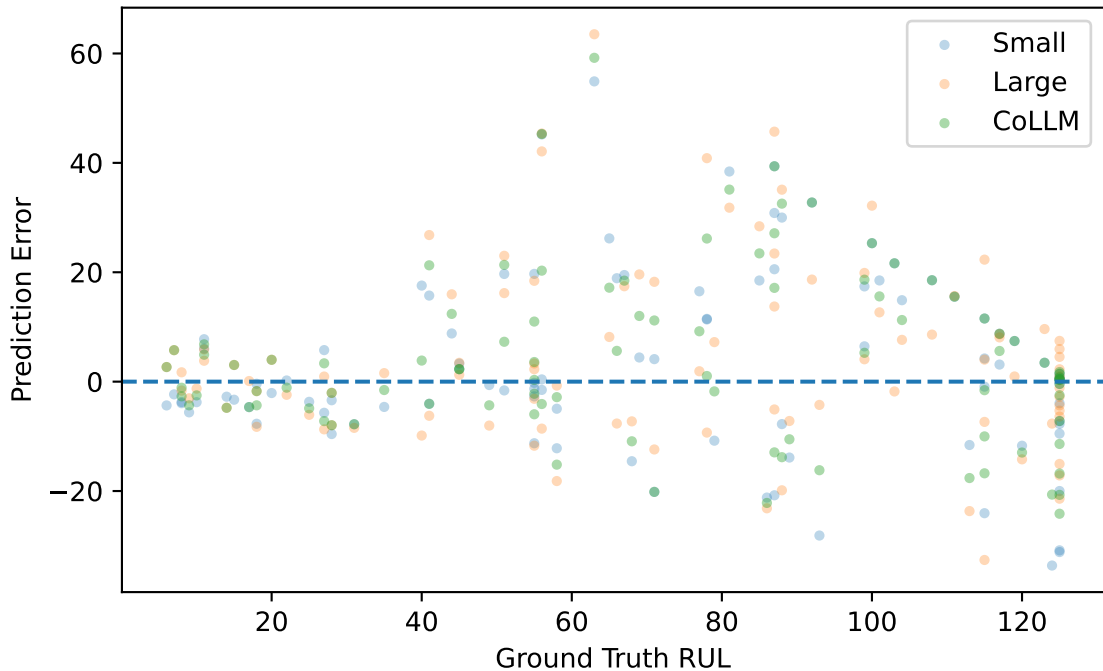
Prediction Error vs RUL (Test Set)
