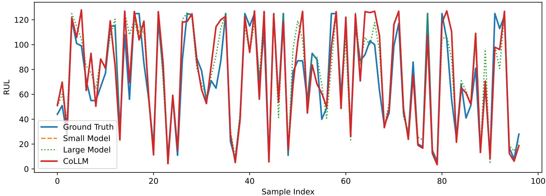
RUL Prediction on Test Set (FD003)
