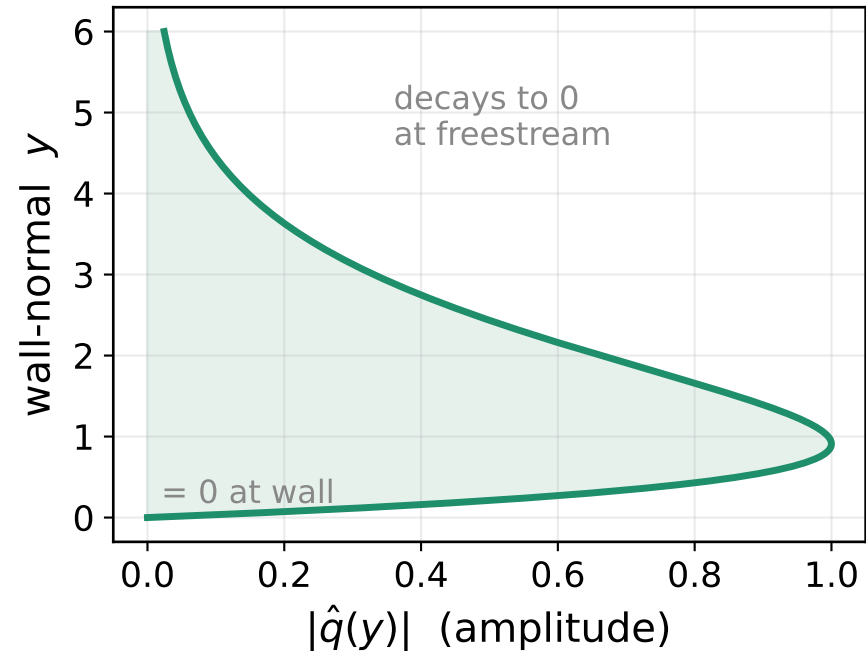
Eigenfunction \hat{q}(y)
