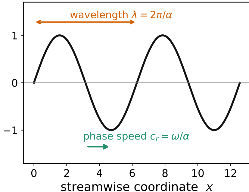
Travelling wave e^{i(\alpha x - \omega t)}
