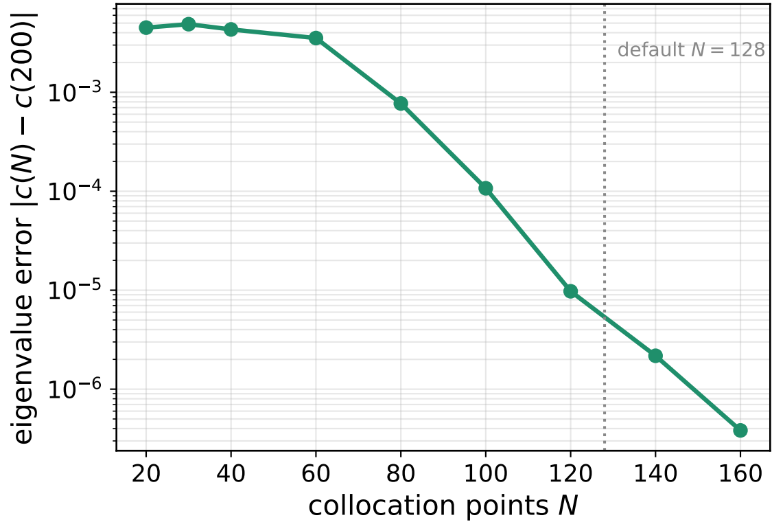
Spectral (exponential) convergence of the Mack-mode eigenvalue
