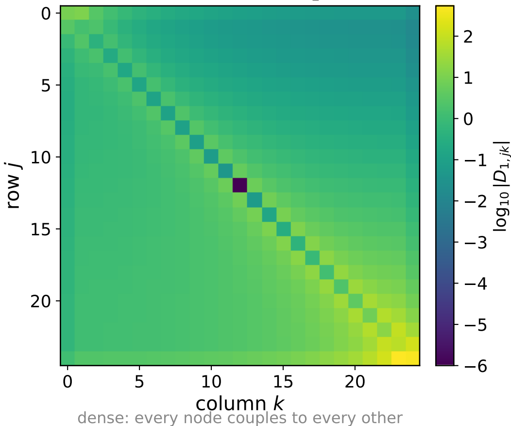
First-derivative matrix D_1 ( 25 \times 25 )
