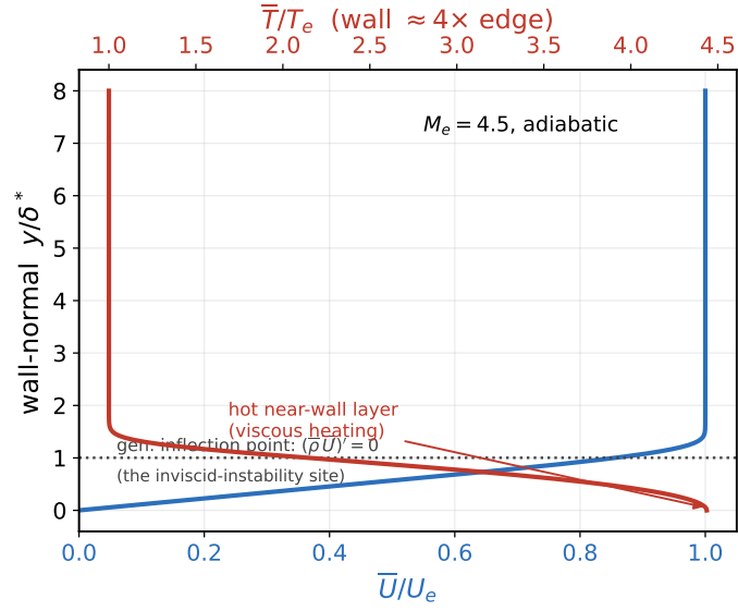
Figure 2: A computed compressible base flow ( M_e = 4.5 , adiabatic). \bar{U}(y)/U_e rises monotonically to the edge; \bar{T}(y) bulges near the wall from viscous heating. These curves and their y -derivatives are the known coefficients \bar{U}, \bar{T}, \dots in the disturbance equations. The dotted line marks the generalised inflection point, the seat of the inviscid instability (discussed in the companion notes on the instability mechanisms).
