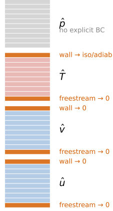
Figure 4: The boundary conditions as row replacement: the stacked state [\hat{u}; \hat{v}; \hat{T}; \hat{p}] with the six overwritten rows highlighted (wall and freestream for \hat{u}, \hat{v}, \hat{T} ); \hat{p} carries no boundary row. Note index 0 is the freestream and n-1 the wall.
