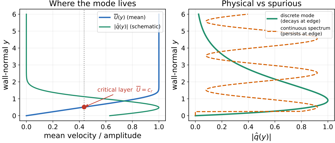
Figure 7: Left: the critical layer is where \bar{U}(y) = c_r ; the mode's amplitude |\hat{q}(y)| tends to peak near it. Right: a discrete boundary-layer mode (solid) decays toward the freestream, while a continuous-spectrum mode (dashed) keeps oscillating to the edge — the basis for the two acceptance tests.
