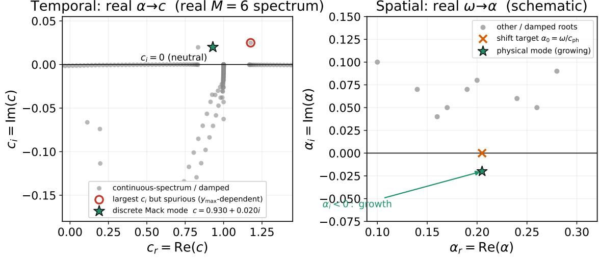
Figure 5: Where the eigenvalues live. Left (temporal): input real \alpha ; the phase speeds c populate the complex plane; the physical discrete mode sits above the line c_i = \text{Im}(c) = 0 (unstable) while the continuous spectrum is damped. Right (spatial, explained in §4): input real \omega ; the wavenumbers \alpha are sought near a shift target \alpha_0 ; the physical mode has \alpha_i < 0 , i.e. growth.
