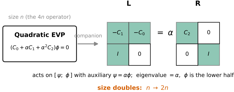
Figure 6: Companion linearisation (11): the 4n -sized quadratic problem becomes an ordinary generalised problem of size 8n in [\psi; \phi] , with \psi = \alpha\phi . Its eigenvalue is exactly \alpha ; the eigenfunction is the lower half.
