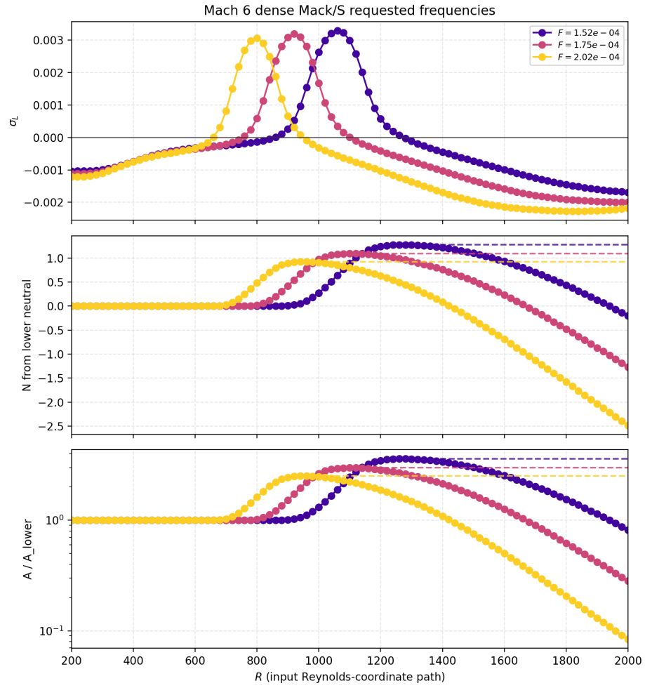
Figure 17: Mach 6 spatial growth rate and integrated N -factor from pyMack — the envelope quantity used for transition estimation.
