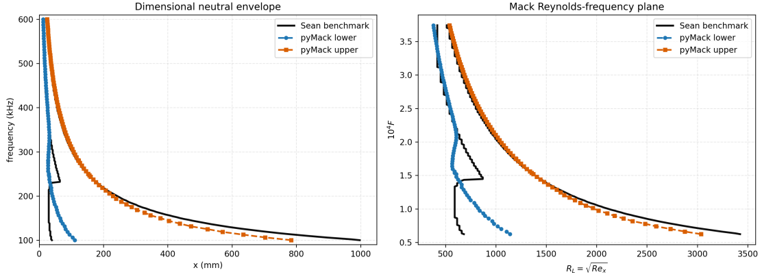
Figure 15: Mach 5.35 nitrogen: pyMack’s neutral branches over the collaborator’s independent LST code. Upper-branch MAE 3.21 mm, lower-branch MAE 1.29 mm (gated bands).
