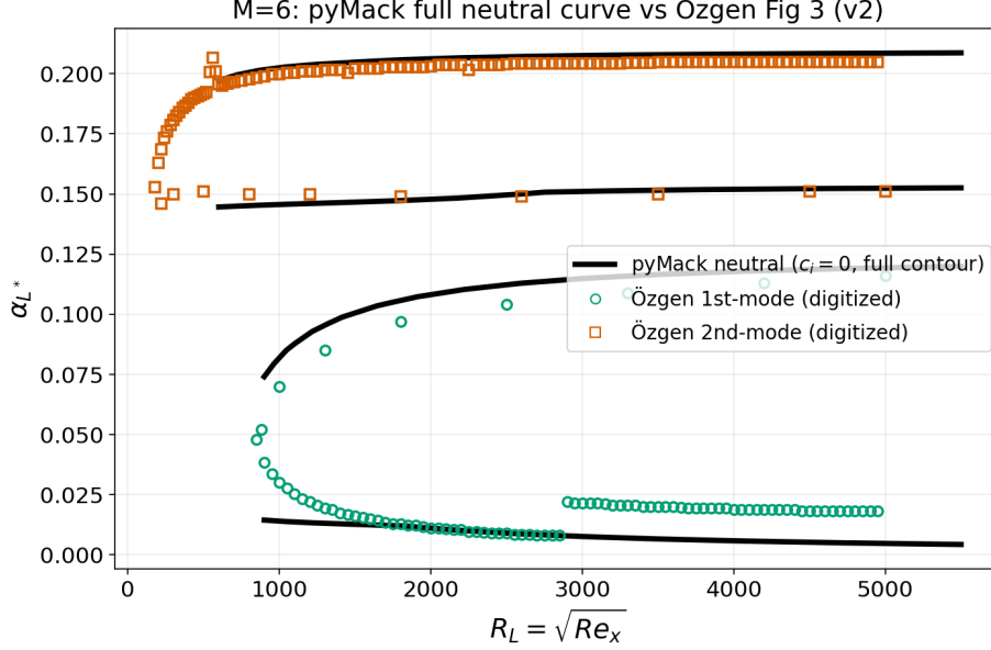
Figure 8: Özgen M = 6 ( acceptable ): four branches; second-mode upper/lower 2/3 % and first cutoff 9 % agree, only the deep low- \alpha first-mode onset (50 %) is extraction-limited.
