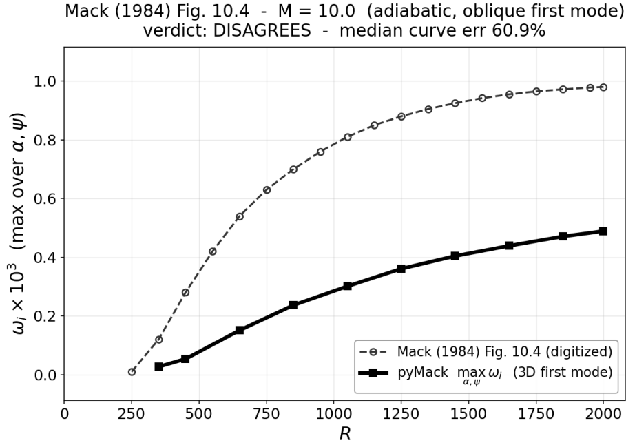
Figure 13: Mack (1984) Fig. 10.4, M = 10 ( disagrees ): curve median 60.9% — the first-mode under-amplification is largest at the top of the Mach range (lower-confidence magnitude, see text).
