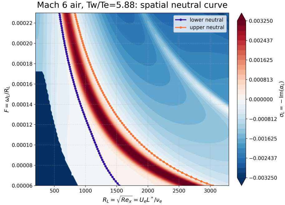
Figure 16: Mach 6 spatial neutral curve produced by pyMack — the second-mode instability boundary in the frequency/streamwise plane, at a representative Mach 6 flat-plate condition ( T_w/T_e = 5.88 ).
