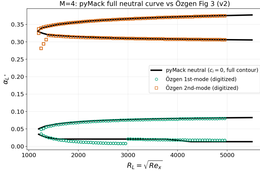
Figure 6: Özgen & Kırcah (2008) Fig. 3, M = 4 ( agrees ): pyMack reproduces the entire two-lobe neutral structure — both second-mode branches at the digitisation floor and the first-mode cutoff to 2%.
