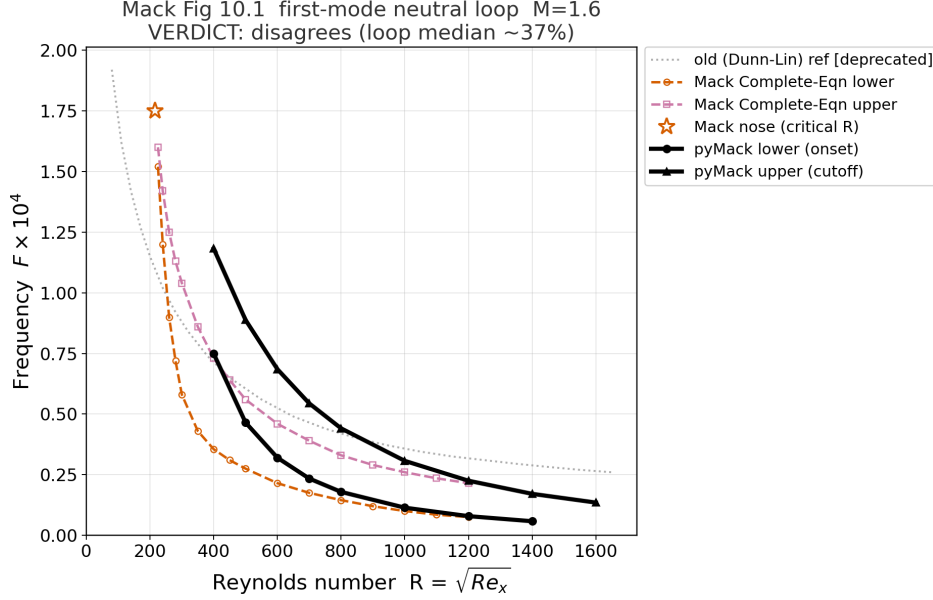
Figure 9: Mack (1984) Fig. 10.1, M = 1.6 ( disagrees ): pyMack’s first-mode neutral loop is wider/higher than Mack’s Complete-Equations loop; critical R \approx 400 vs. Mack’s \sim 215 .
