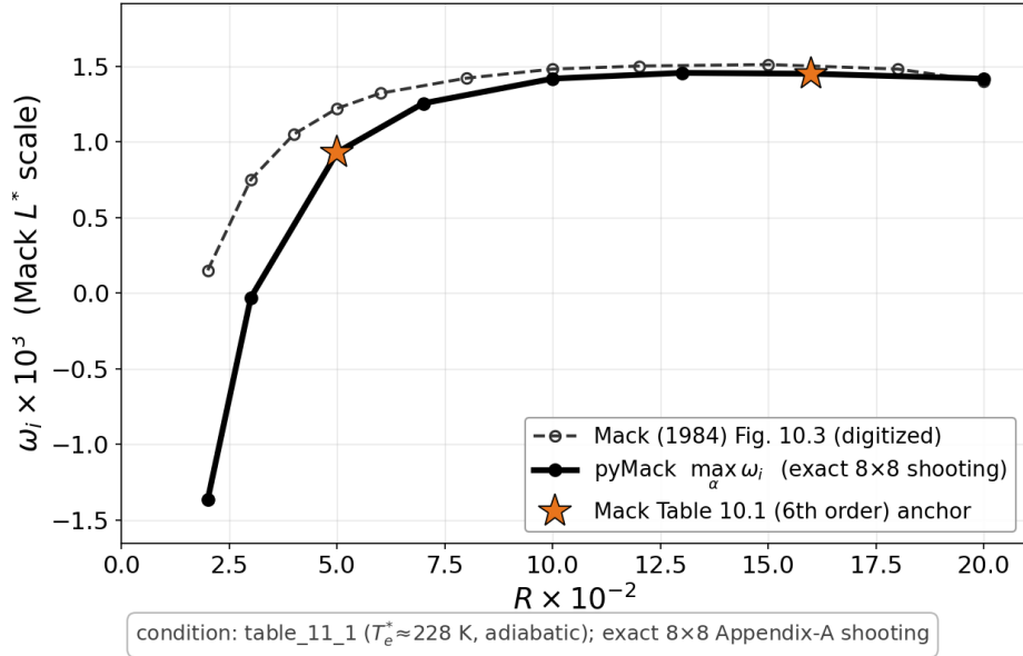
Mack (1984) Fig. 10.3 overlay - M = 1.3 , \psi = 45^\circ first mode verdict: AGREES - median curve err 3.8%, Table-10.1 anchor 0.9%
