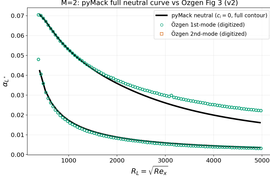
Figure 7: Özgen M = 2 ( acceptable ): both first-mode branches over the full R -range by eigenvalue continuation (lower 7 %, upper 8 %).
