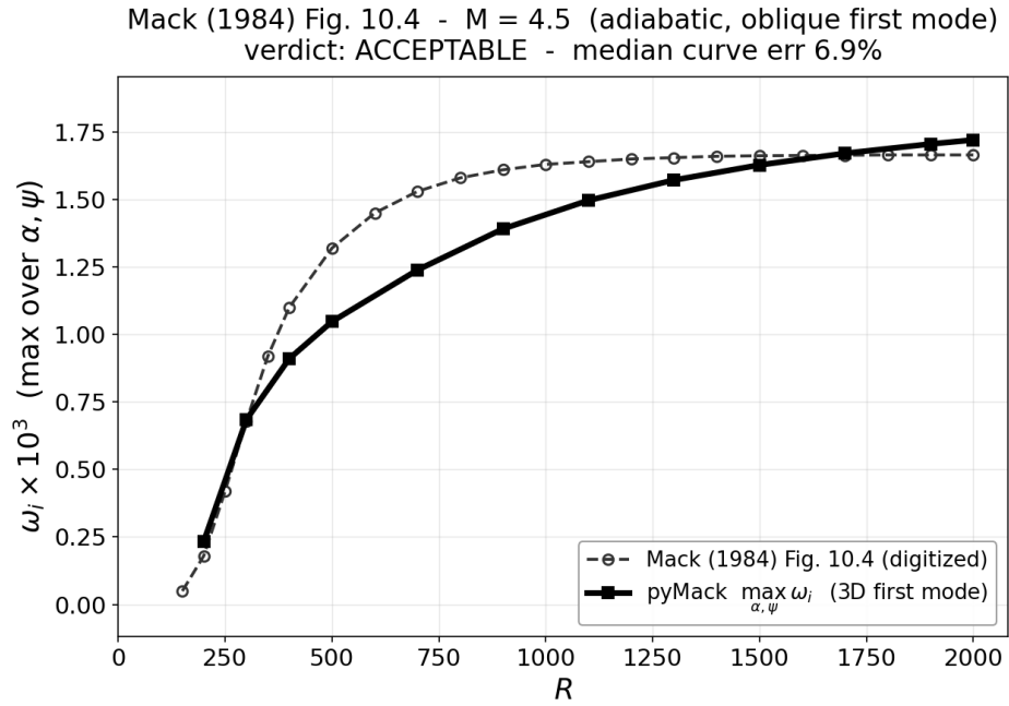
Figure 12: Mack (1984) Fig. 10.4, M = 4.5 ( acceptable ): oblique first mode optimised over (\alpha, \psi) , curve median 6.9%.
