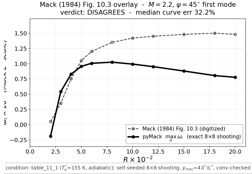
Figure 11: Mack (1984) Fig. 10.3, M = 2.2 , \psi = 45^\circ ( disagrees ): correct topology but curve median 32.2% — the first-mode under-amplification, confirmed convergence-stable.
