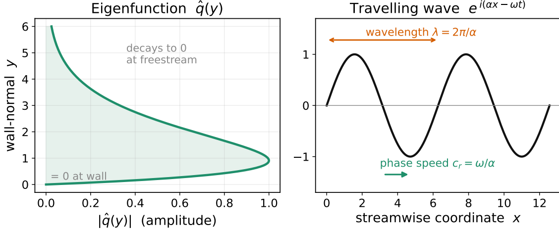
Figure 5: The ansatz (6) factorises a disturbance q' = \hat{q}(y) e^{i(\alpha x - \omega t)} into a wall-normal shape \hat{q}(y) (left; zero at the wall, decaying at the edge — the eigenfunction) times a travelling wave in x (right; wavelength 2\pi/\alpha , phase speed c_r = \text{Re}(c) ).
