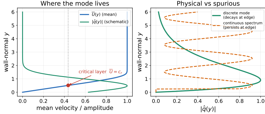
Figure 6: The critical layer (left panel): the wall-normal location where the mean velocity \bar{U}(y) crosses the phase speed c_r , at which the eigenfunction |\hat{q}(y)| typically peaks. (The right panel, discrete-vs-spurious mode classification, is discussed in the companion Numerical Methods note.)
