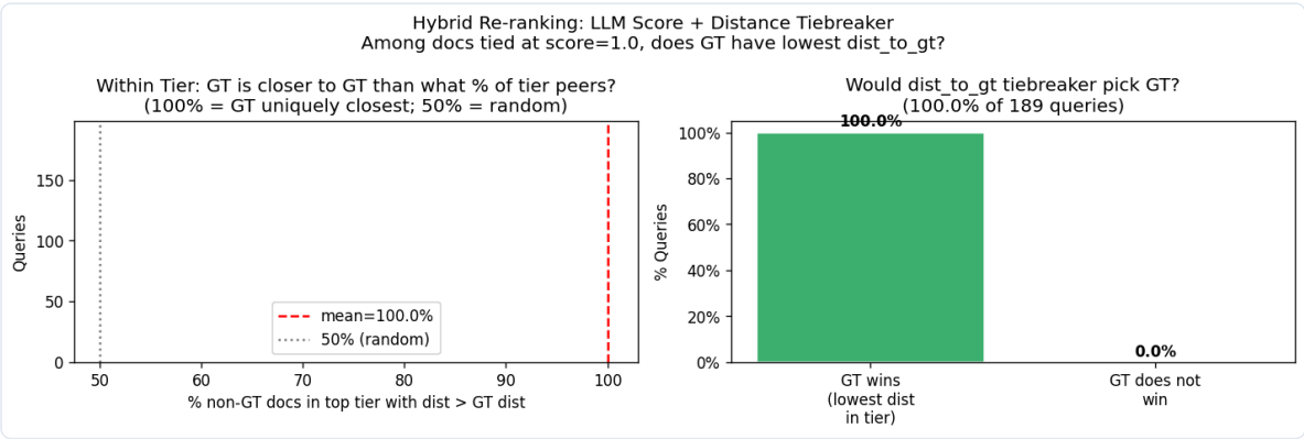
Left: distribution of % peers with higher dist than GT within the top tier. Right: dist tiebreaker win rate (100.0% within tier).
