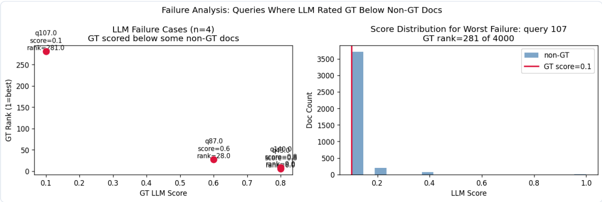
GT rank and score for each failure case. Right: score distribution for the worst failure (query 107).
