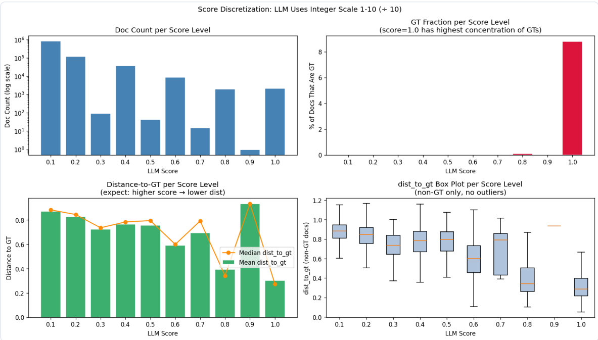
Score level breakdown: doc counts (log scale), GT fraction, distance distributions, and box plots per score level.
