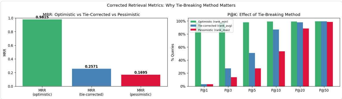
Effect of tie-breaking method on MRR and P@K. Green = optimistic (rank_min), blue = tie-corrected (rank_avg), red = pessimistic (rank_max).
