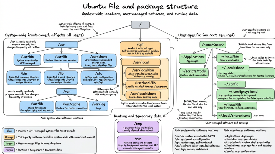
Figure 3.1.: Detailed structure of Ubuntu package layout
