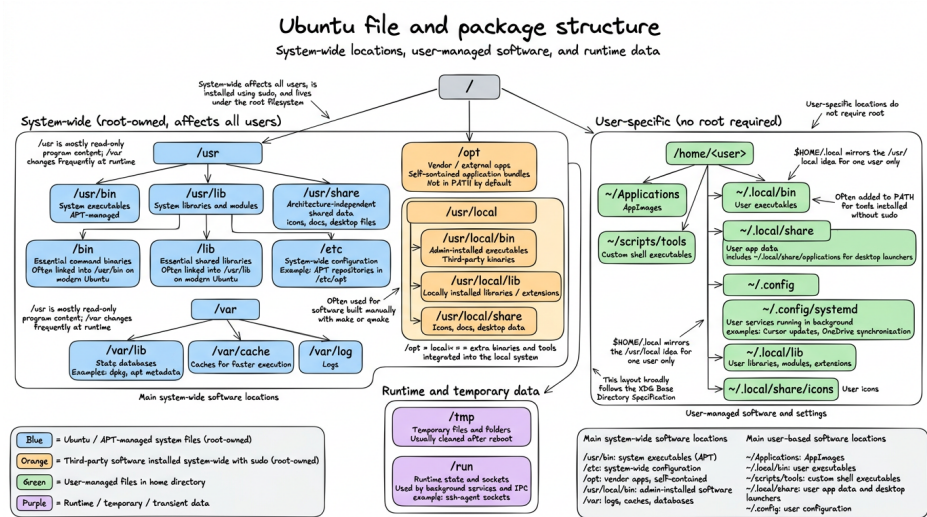
Figure 2.1: Detailed structure of Ubuntu package layout
