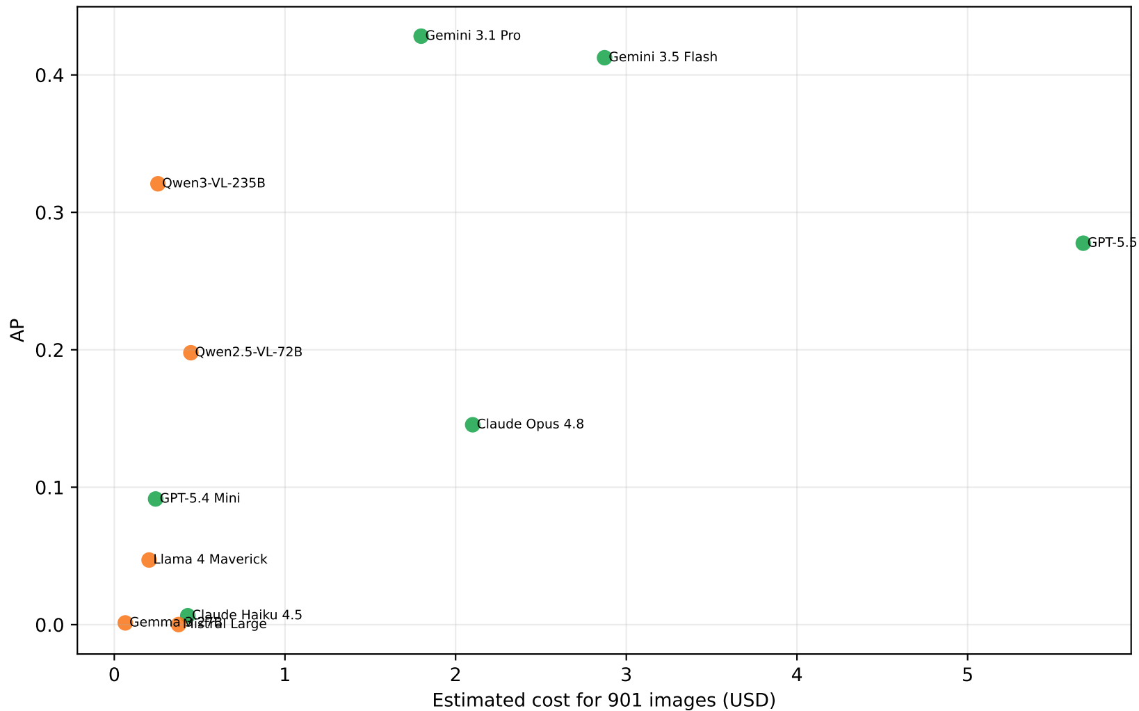
COCO-unseen API refresh: cost vs AP
