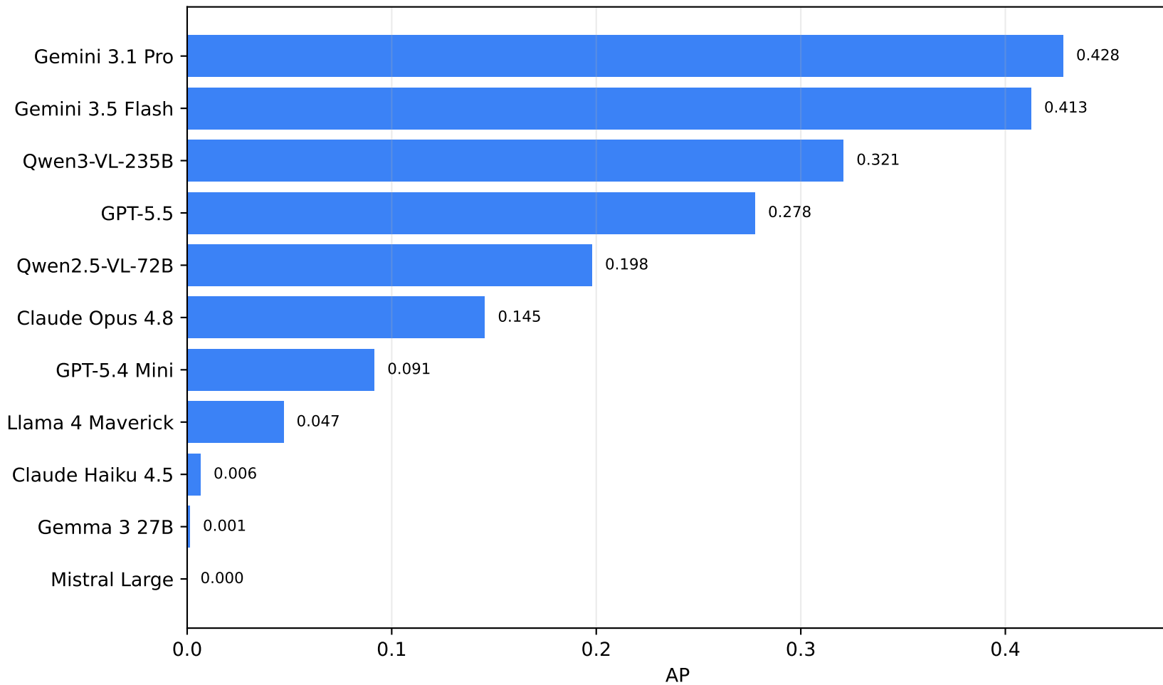
COCO-unseen API refresh: AP
