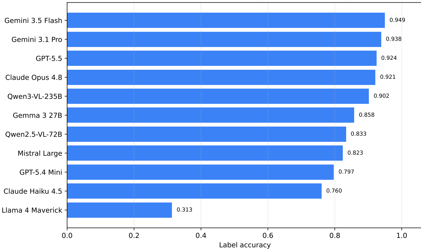
COCO-unseen API refresh: dynamic-label accuracy
