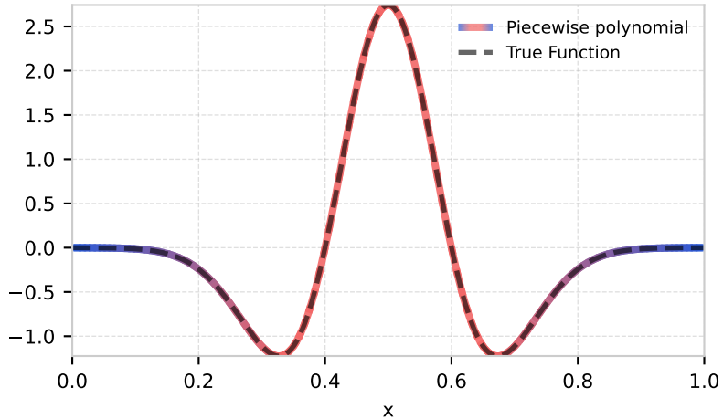
Piecewise Polynomial Approximation
