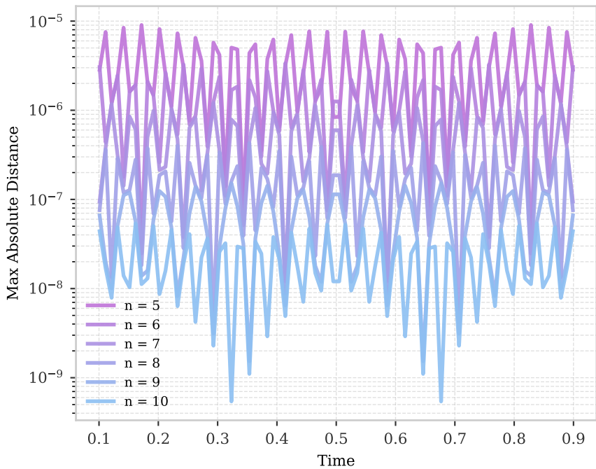
Linearized Time Evolution
