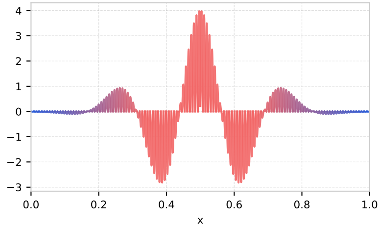
Approximation Error
