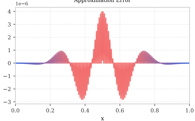
Approximation Error
