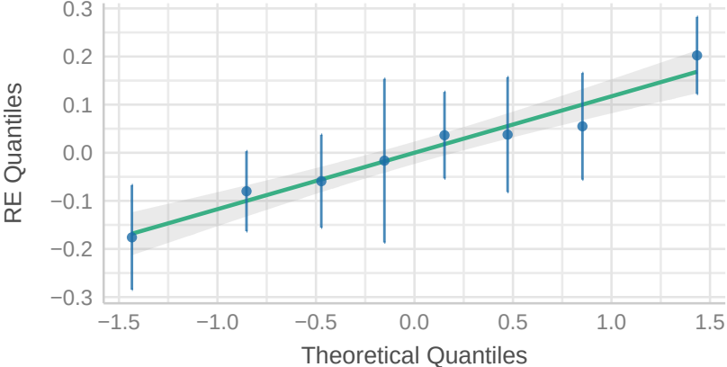
Normality of Random Effects (Site) Dots should be plotted along the line
