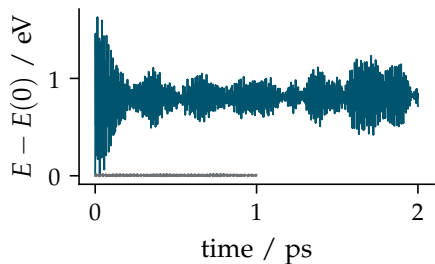
(c) wrong units
