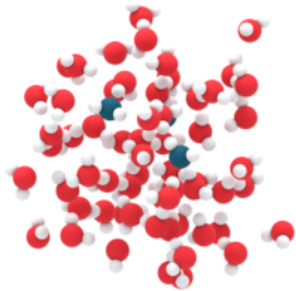
(a) 0 ps
