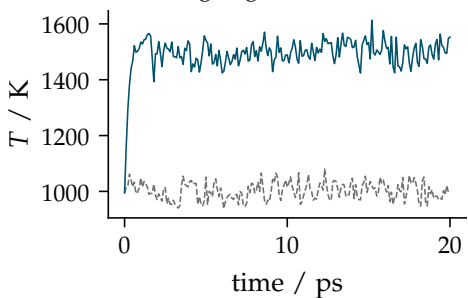
(e) wrong degrees of freedom
