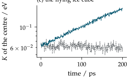
(c) the flying ice cube
