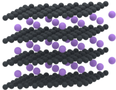
(b) \text{LiC}_6 , sheets 3.70 Å apart
