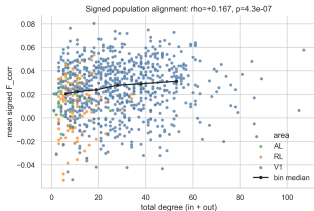
H7: signed F_{\text{corr}} association is weak and layer-sensitive
