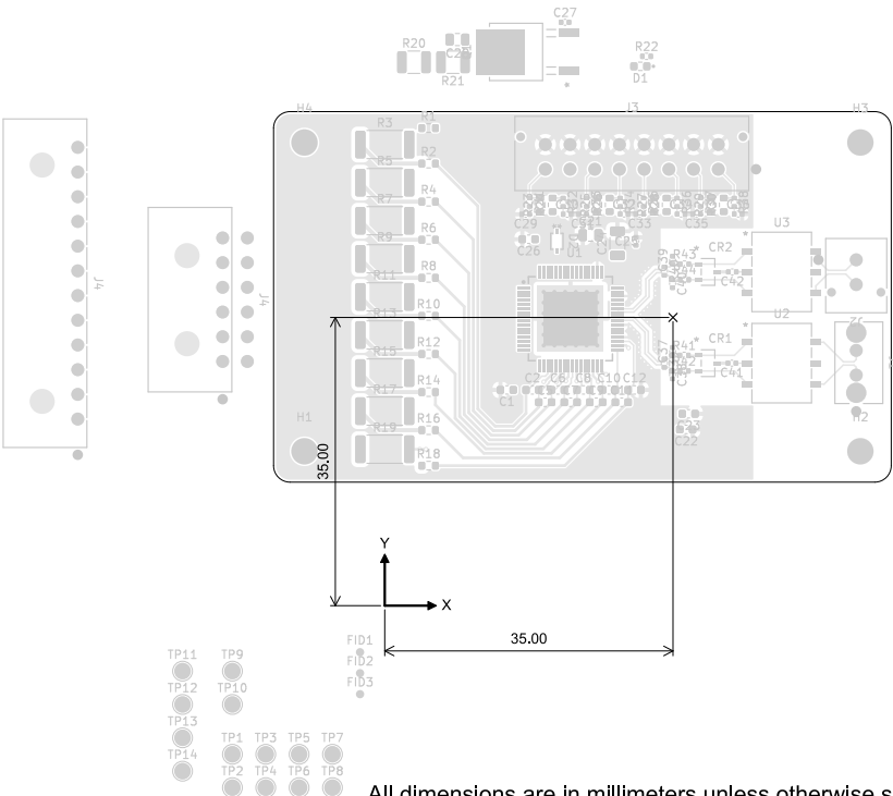
Top Test Points (Scale 1:1)
