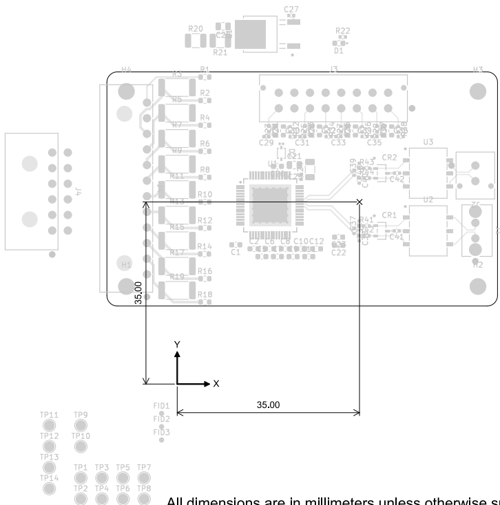
Top Test Points (Scale 1:1)
