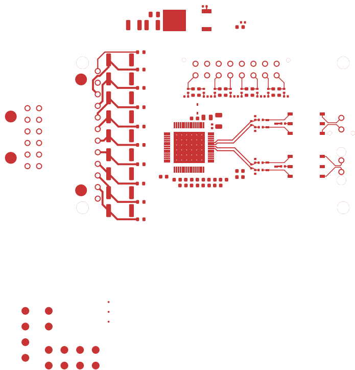
L1 (Sig, PWR) (Scale 1:1)
