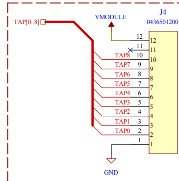
Cell Balance Connector
