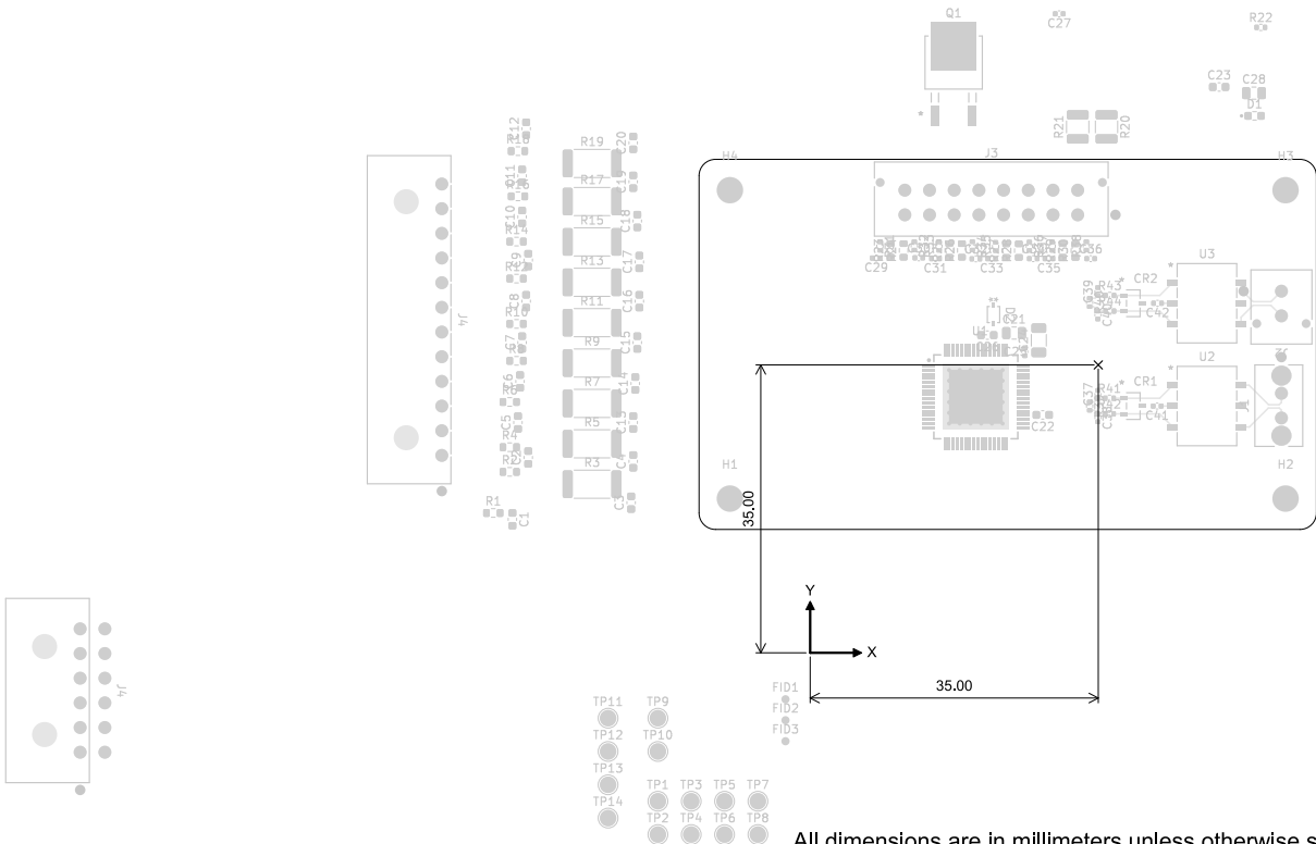
Top Test Points (Scale 1:1)
