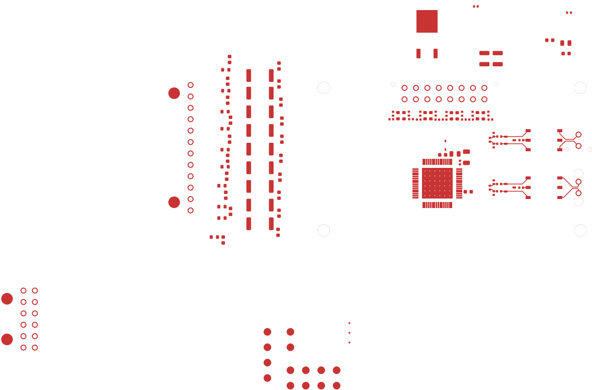
L1 (Sig, PWR) (Scale 1:1)
