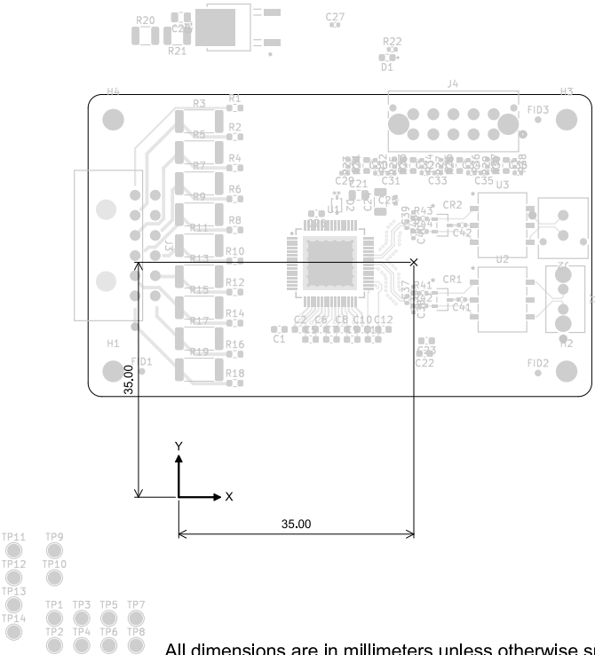
Top Test Points (Scale 1:1)
