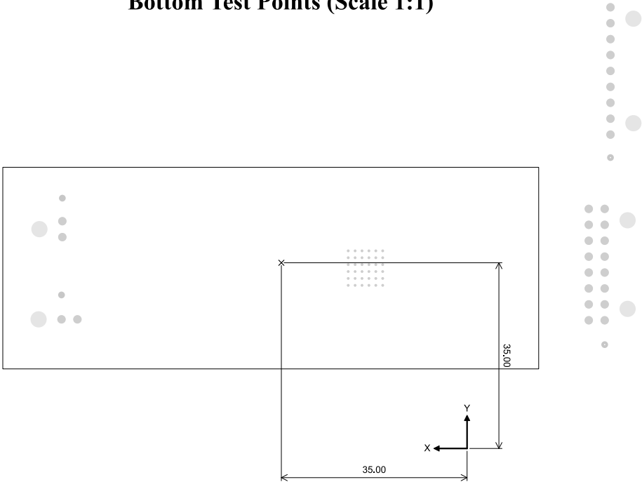
Bottom Test Points (Scale 1:1)
