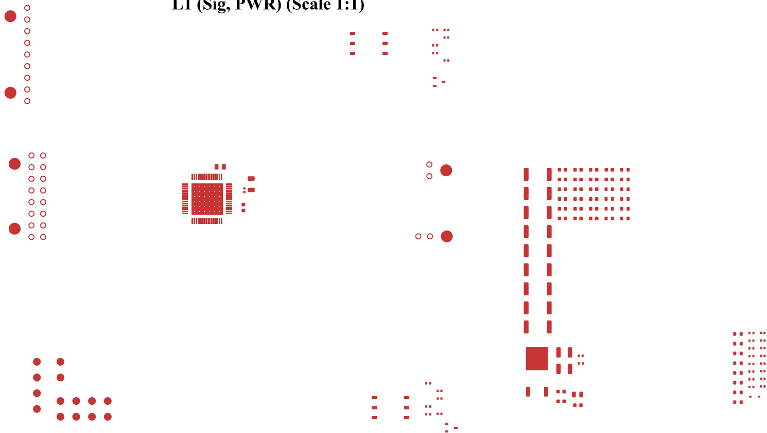
L1 (Sig, PWR) (Scale 1:1)
