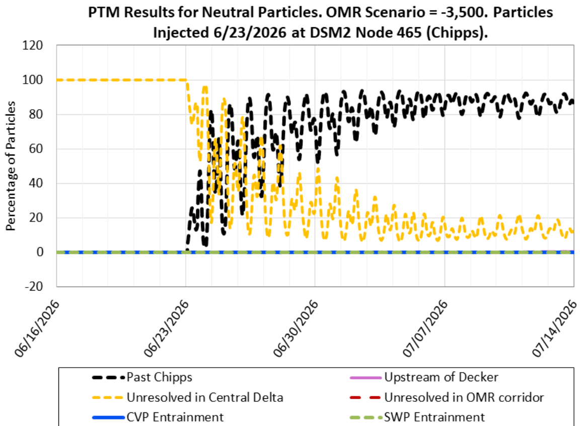
Figure 10: PTM Results for Neutral Particles. OMR Scenario -3,500 cfs. Particles Injected 06/23/2026 at DSM2 Node 465 (Chippis)
