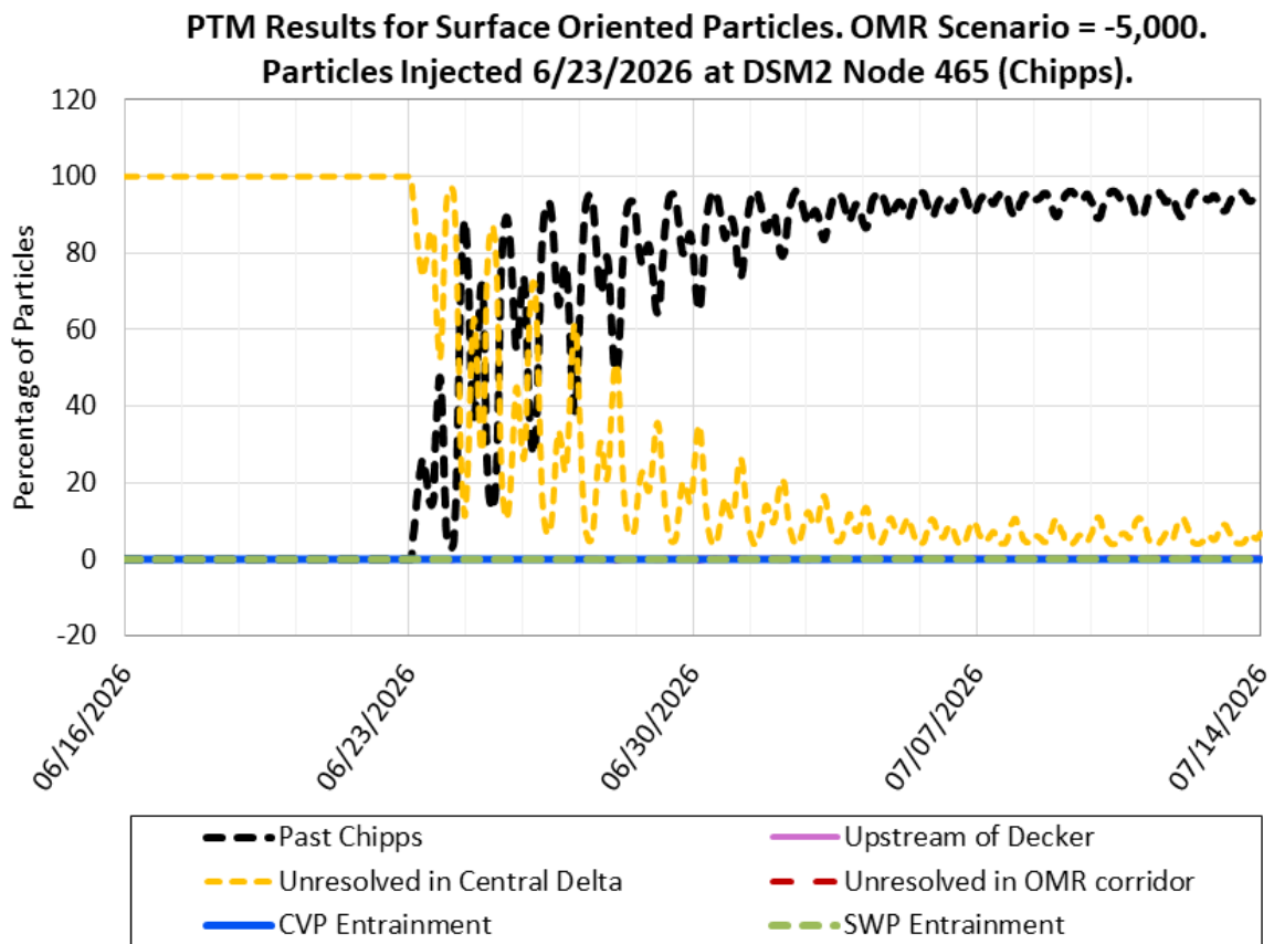
Figure 21: PTM Results for Surface Oriented Particles. OMR Scenario -5,000 cfs. Particles Injected 06/23/2026 at DSM2 Node 465 (Chipps)
