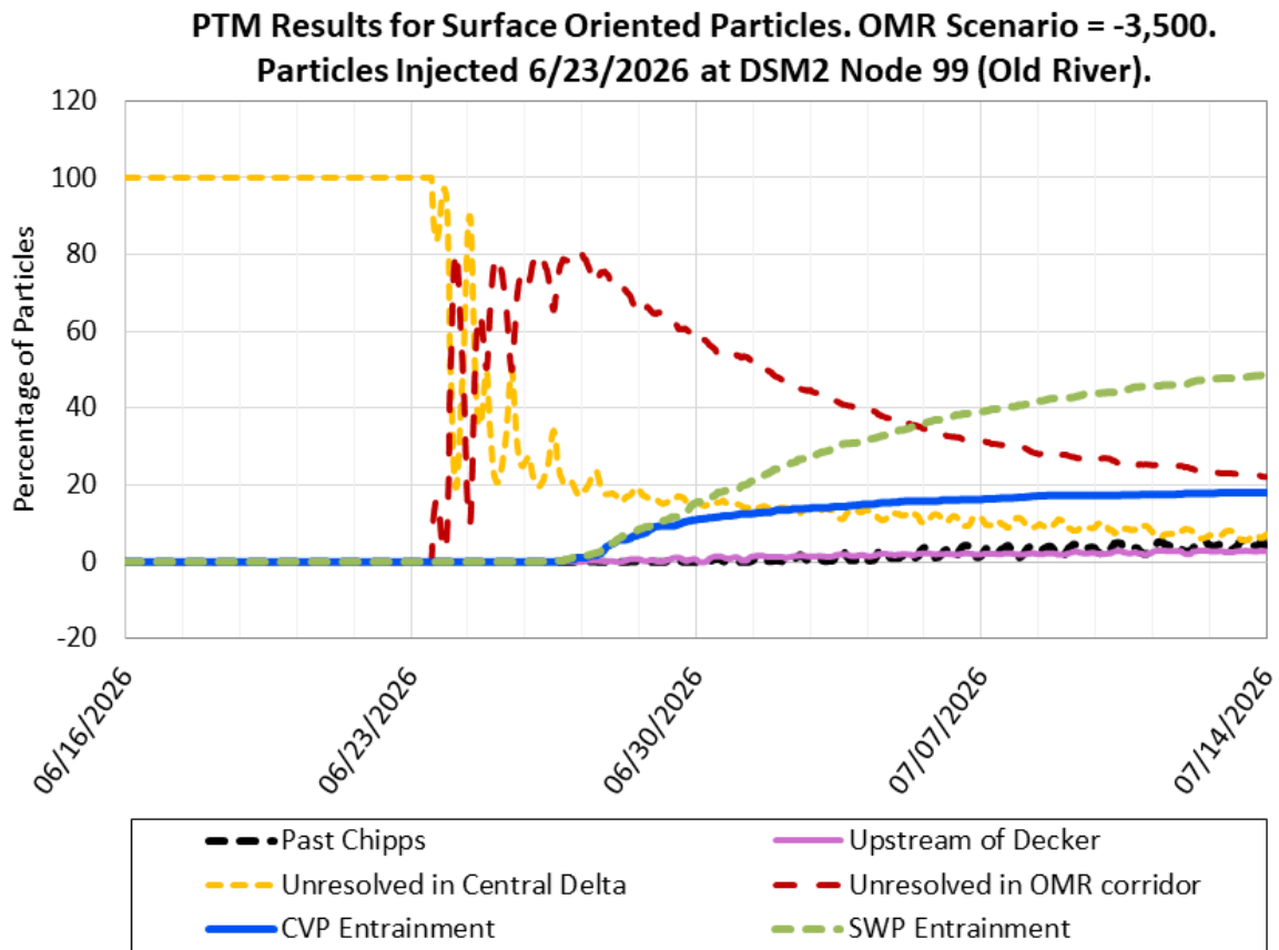
Figure 31: PTM Results for Surface Oriented Particles. OMR Scenario -3,500 cfs. Particles Injected 06/23/2026 at DSM2 Node 99 (Old River)
