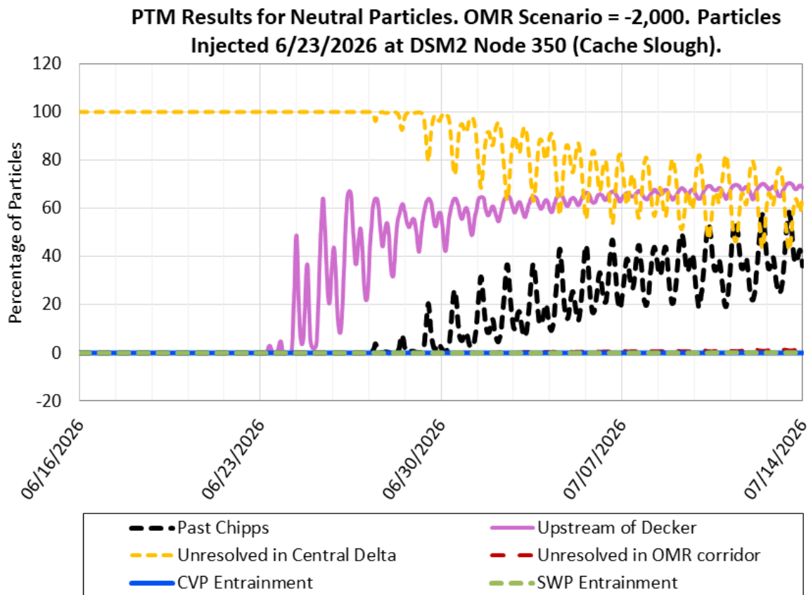
Figure 14: PTM Results for Neutral Particles. OMR Scenario -2,000 cfs. Particles Injected 06/23/2026 at DSM2 Node 350 (Cache Slough)
