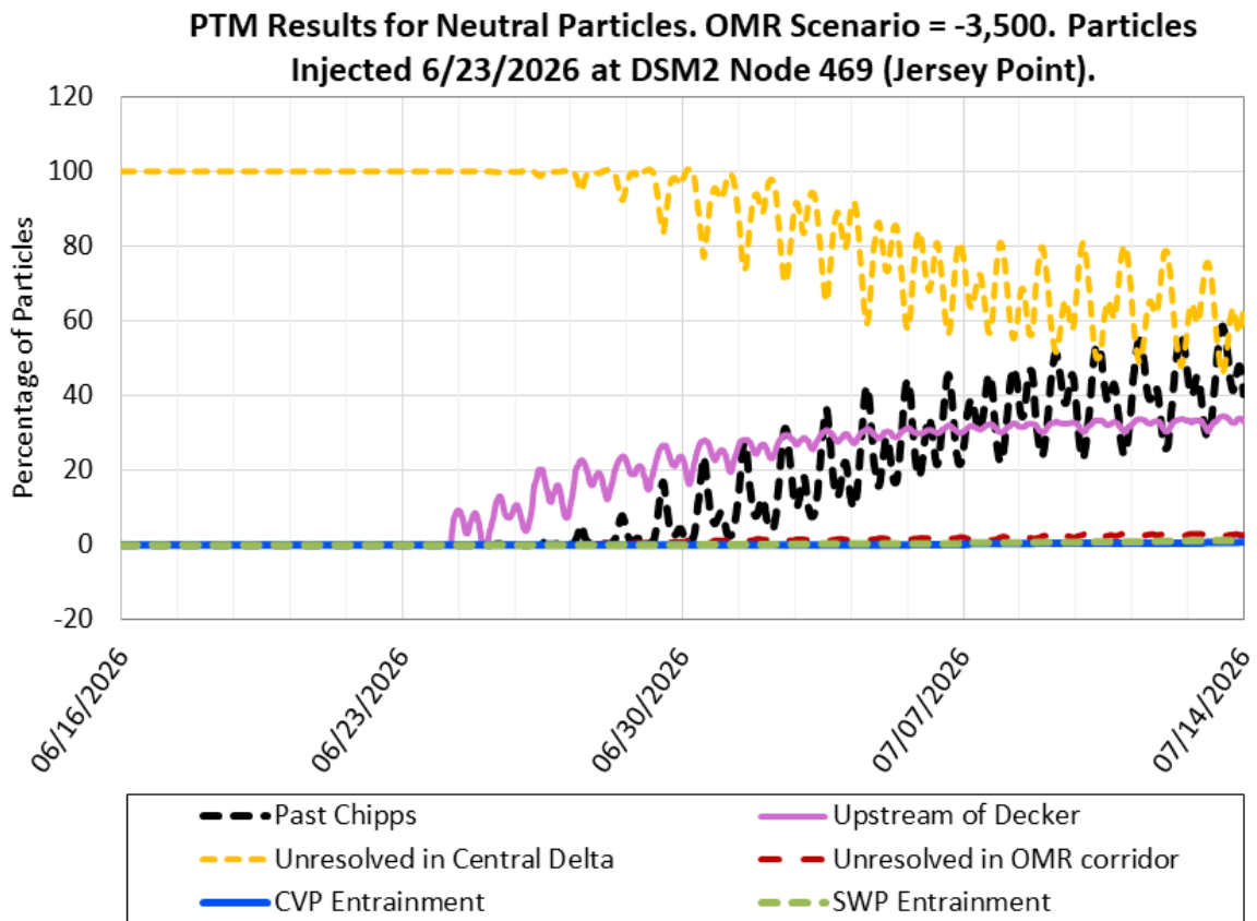
Figure 16: PTM Results for Neutral Particles. OMR Scenario -3,500 cfs. Particles Injected 06/23/2026 at DSM2 Node 469 (Jersey Point)
