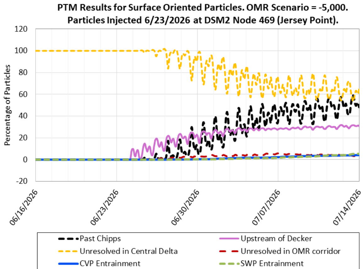
Figure 27: PTM Results for Surface Oriented Particles. OMR Scenario -5,000 cfs. Particles Injected 06/23/2026 at DSM2 Node 469 (Jersey Point)
