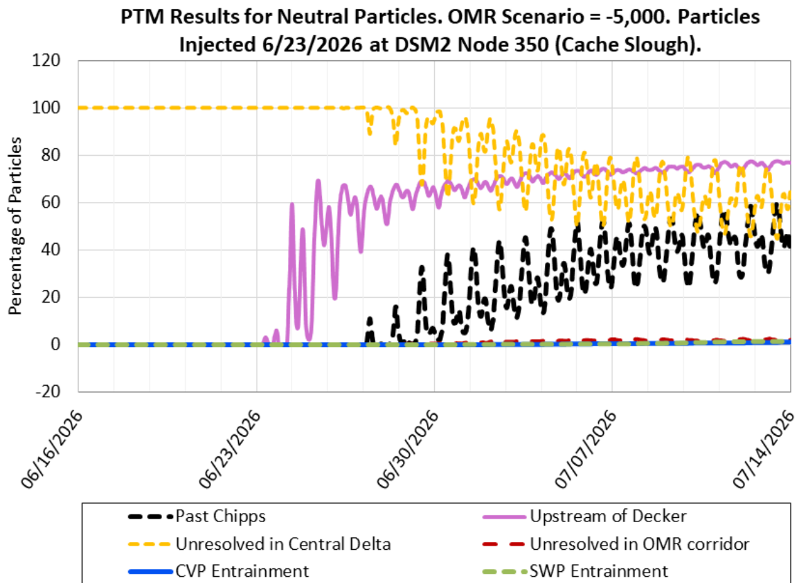
Figure 12: PTM Results for Neutral Particles. OMR Scenario -5,000 cfs. Particles Injected 06/23/2026 at DSM2 Node 350 (Cache Slough)
