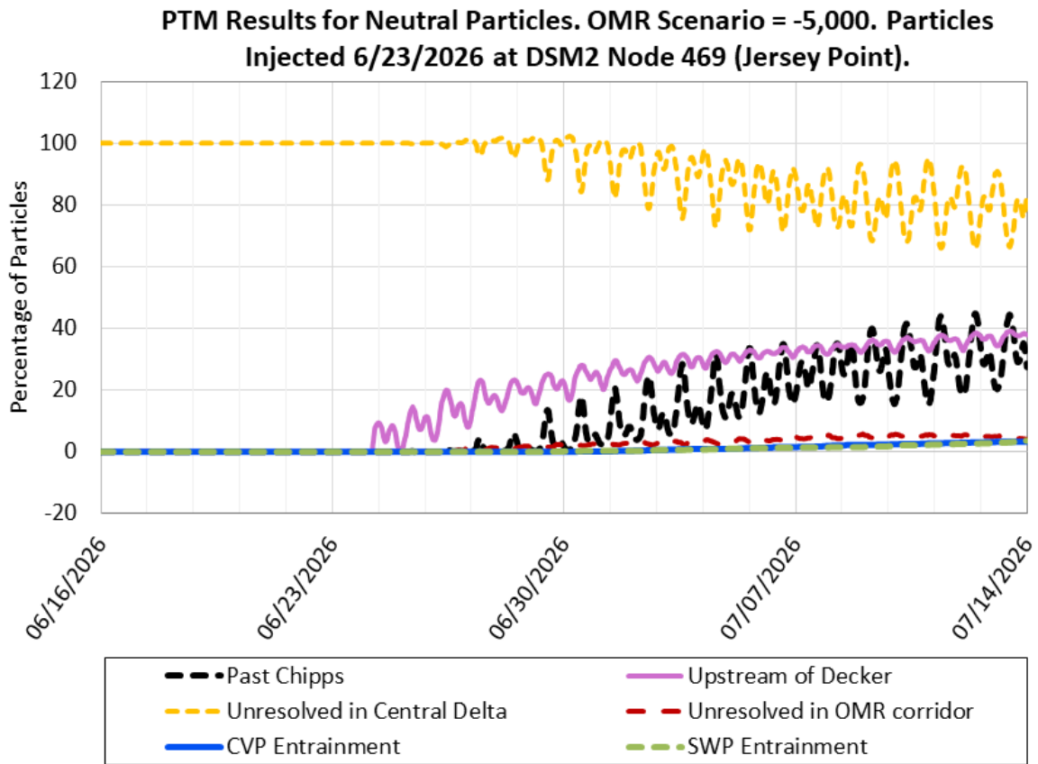
Figure 15: PTM Results for Neutral Particles. OMR Scenario -5,000 cfs. Particles Injected 06/23/2026 at DSM2 Node 469 (Jersey Point)
