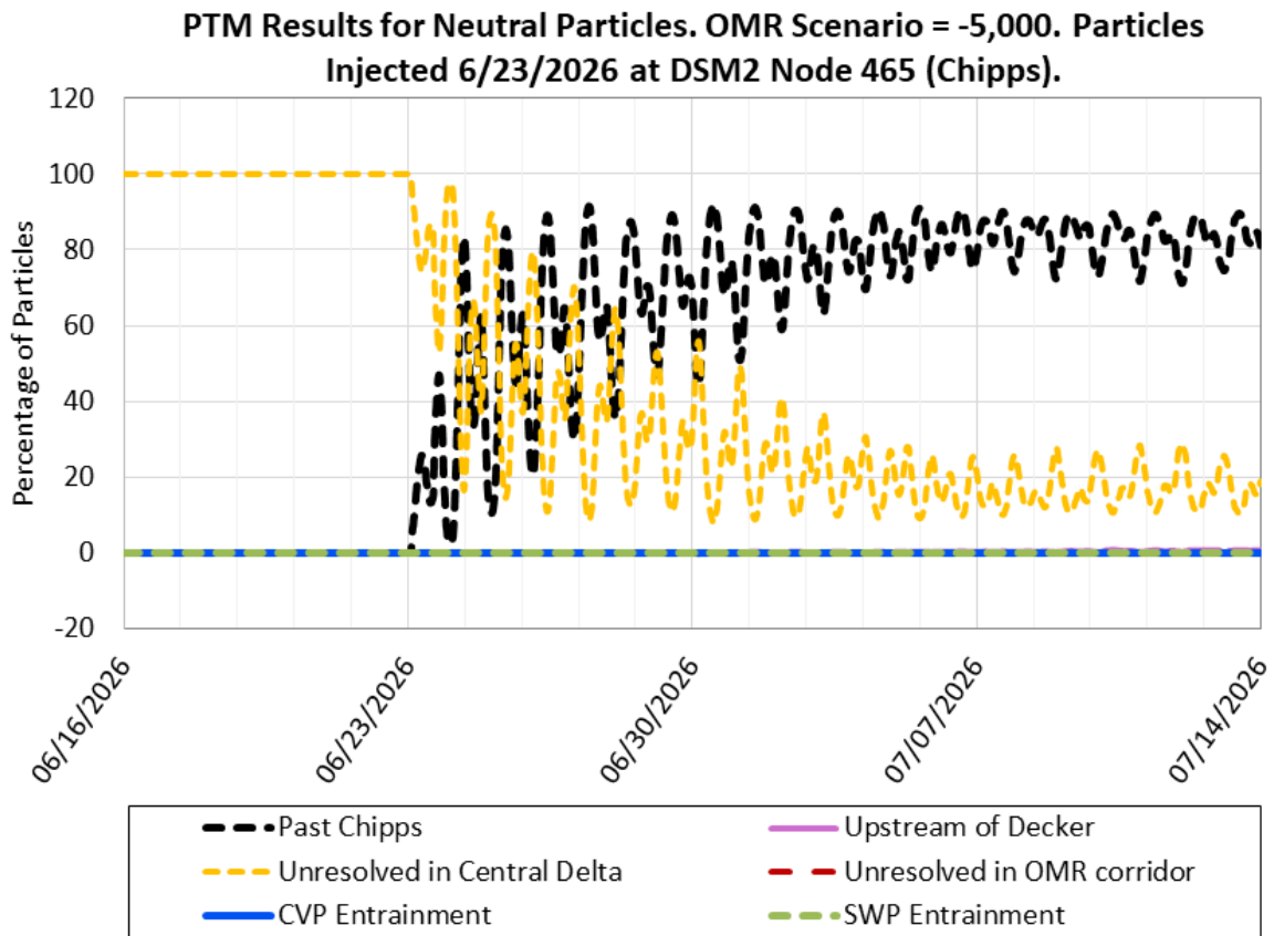
Figure 9: PTM Results for Neutral Particles. OMR Scenario -5,000 cfs. Particles Injected 06/23/2026 at DSM2 Node 465 (Chippis)
