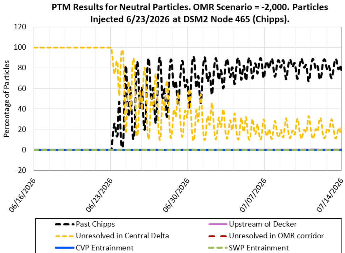
Figure 11: PTM Results for Neutral Particles. OMR Scenario -2,000 cfs. Particles Injected 06/23/2026 at DSM2 Node 465 (Chippis)
