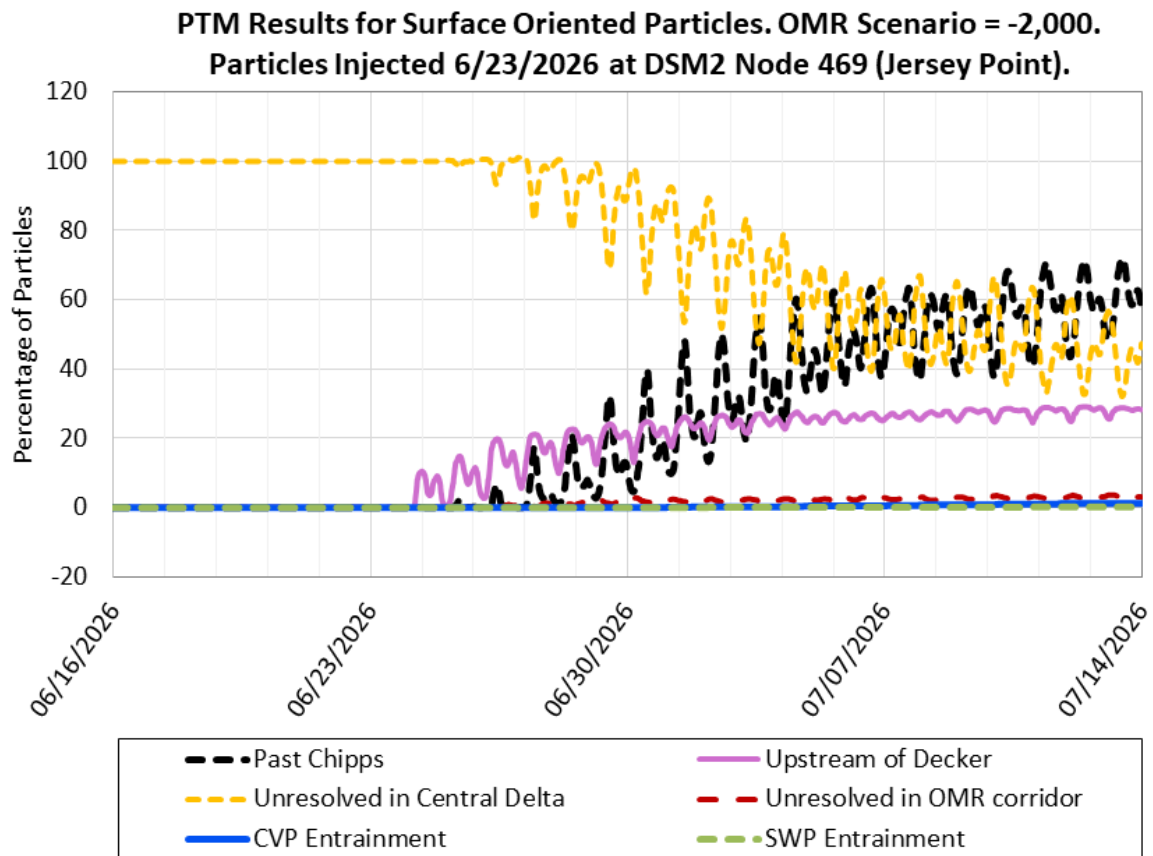
Figure 29: PTM Results for Surface Oriented Particles. OMR Scenario -2,000 cfs. Particles Injected 06/23/2026 at DSM2 Node 469 (Jersey Point)
