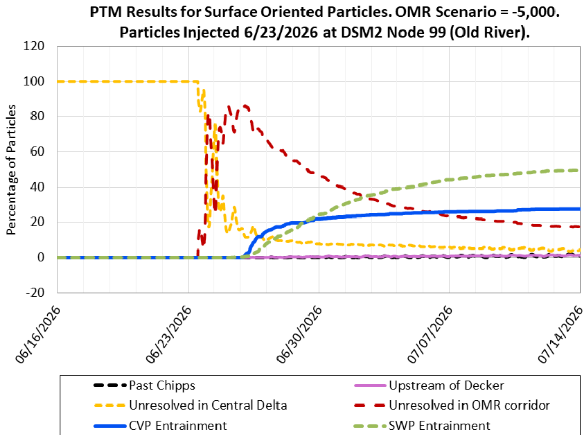
Figure 30: PTM Results for Surface Oriented Particles. OMR Scenario -5,000 cfs. Particles Injected 06/23/2026 at DSM2 Node 99 (Old River)
