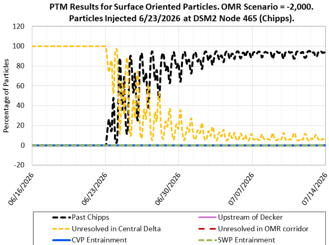
Figure 23: PTM Results for Surface Oriented Particles. OMR Scenario -2,000 cfs. Particles Injected 06/23/2026 at DSM2 Node 465 (Chipps)
