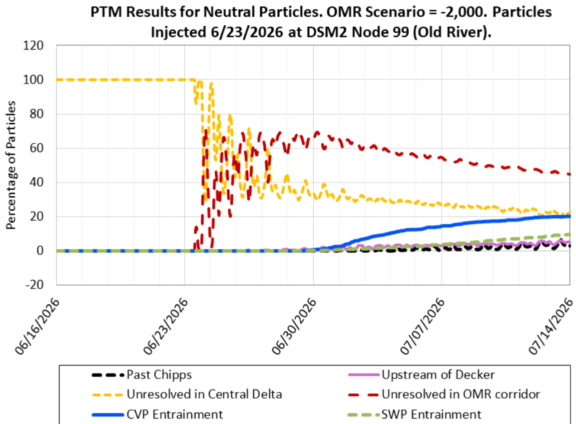
Figure 20: PTM Results for Neutral Particles. OMR Scenario -2,000 cfs. Particles Injected 06/23/2026 at DSM2 Node 99 (Old River)
