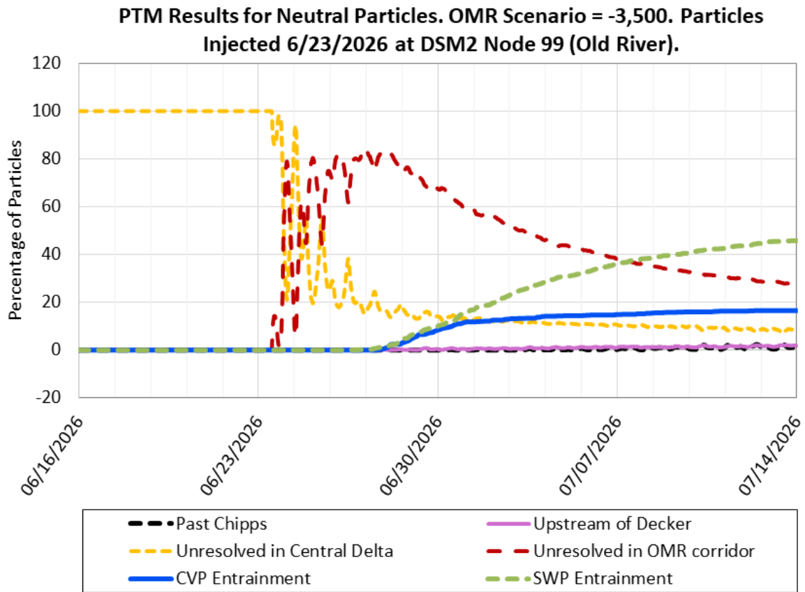
Figure 19: PTM Results for Neutral Particles. OMR Scenario -3,500 cfs. Particles Injected 06/23/2026 at DSM2 Node 99 (Old River)
