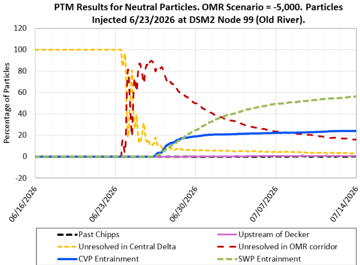
Figure 18: PTM Results for Neutral Particles. OMR Scenario -5,000 cfs. Particles Injected 06/23/2026 at DSM2 Node 99 (Old River)
