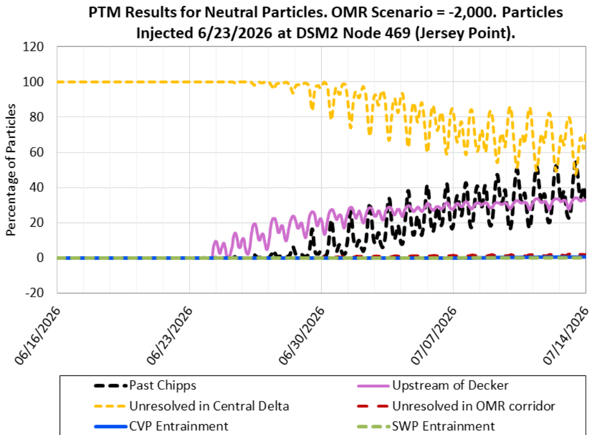
Figure 17: PTM Results for Neutral Particles. OMR Scenario -2,000 cfs. Particles Injected 06/23/2026 at DSM2 Node 469 (Jersey Point)
