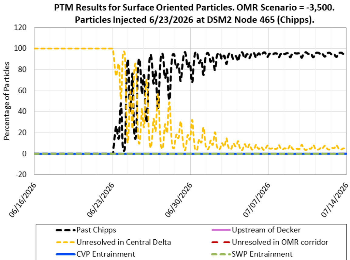
Figure 22: PTM Results for Surface Oriented Particles. OMR Scenario -3,500 cfs. Particles Injected 06/23/2026 at DSM2 Node 465 (Chipps)
