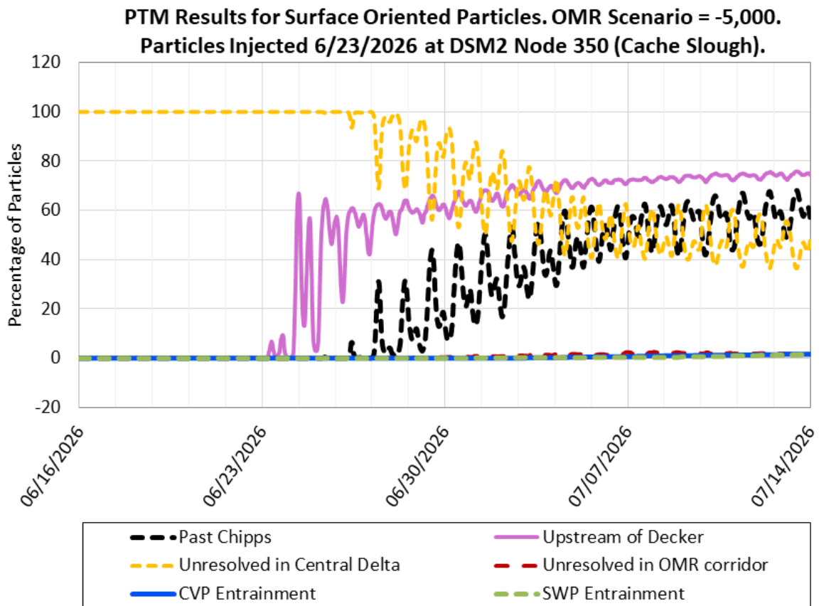
Figure 24: PTM Results for Surface Oriented Particles. OMR Scenario -5,000 cfs. Particles Injected 06/23/2026 at DSM2 Node 350 (Cache Slough)
