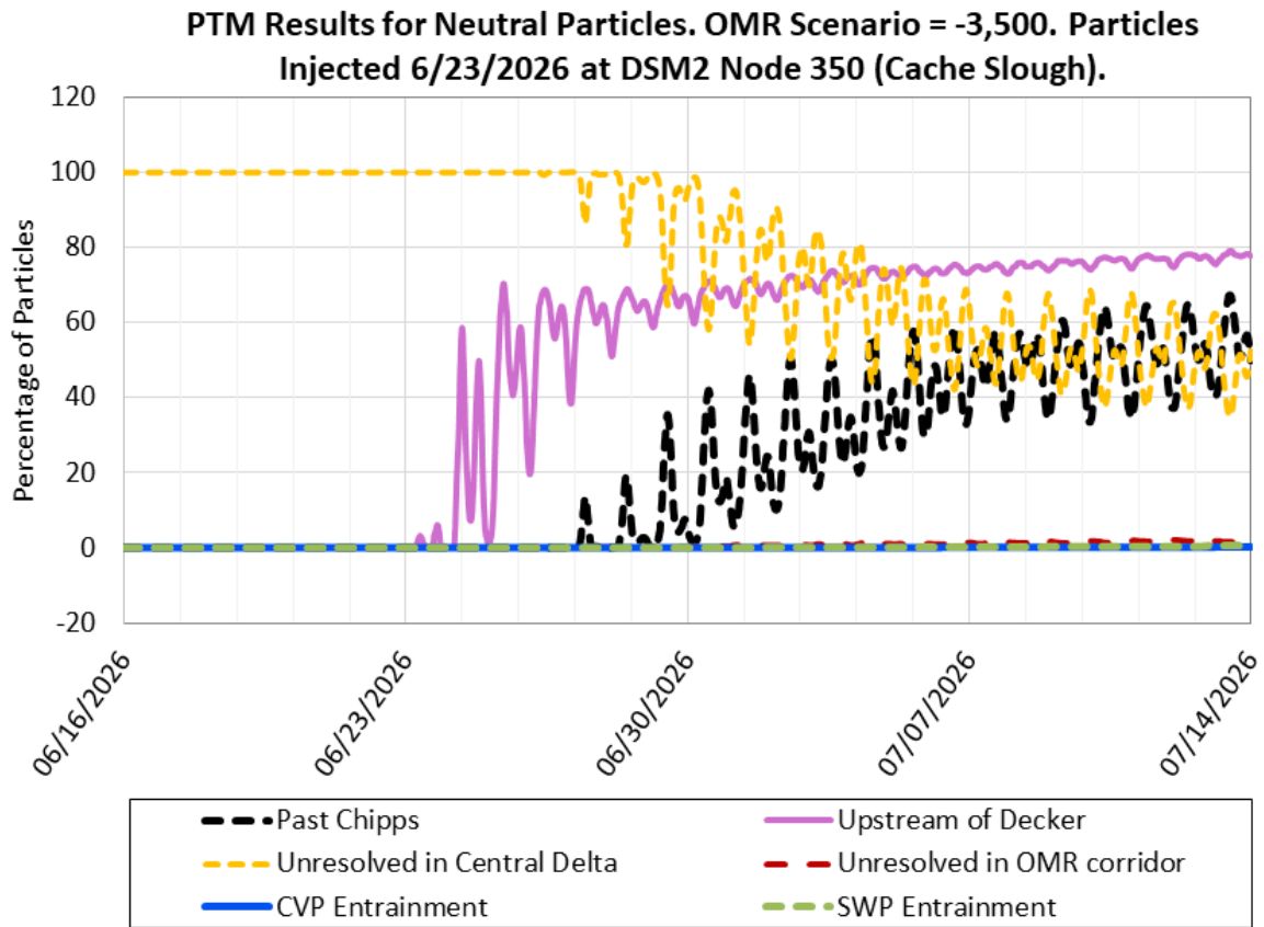
Figure 13: PTM Results for Neutral Particles. OMR Scenario -3,500 cfs. Particles Injected 06/23/2026 at DSM2 Node 350 (Cache Slough)
