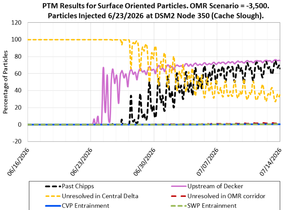
Figure 25: PTM Results for Surface Oriented Particles. OMR Scenario -3,500 cfs. Particles Injected 06/23/2026 at DSM2 Node 350 (Cache Slough)
