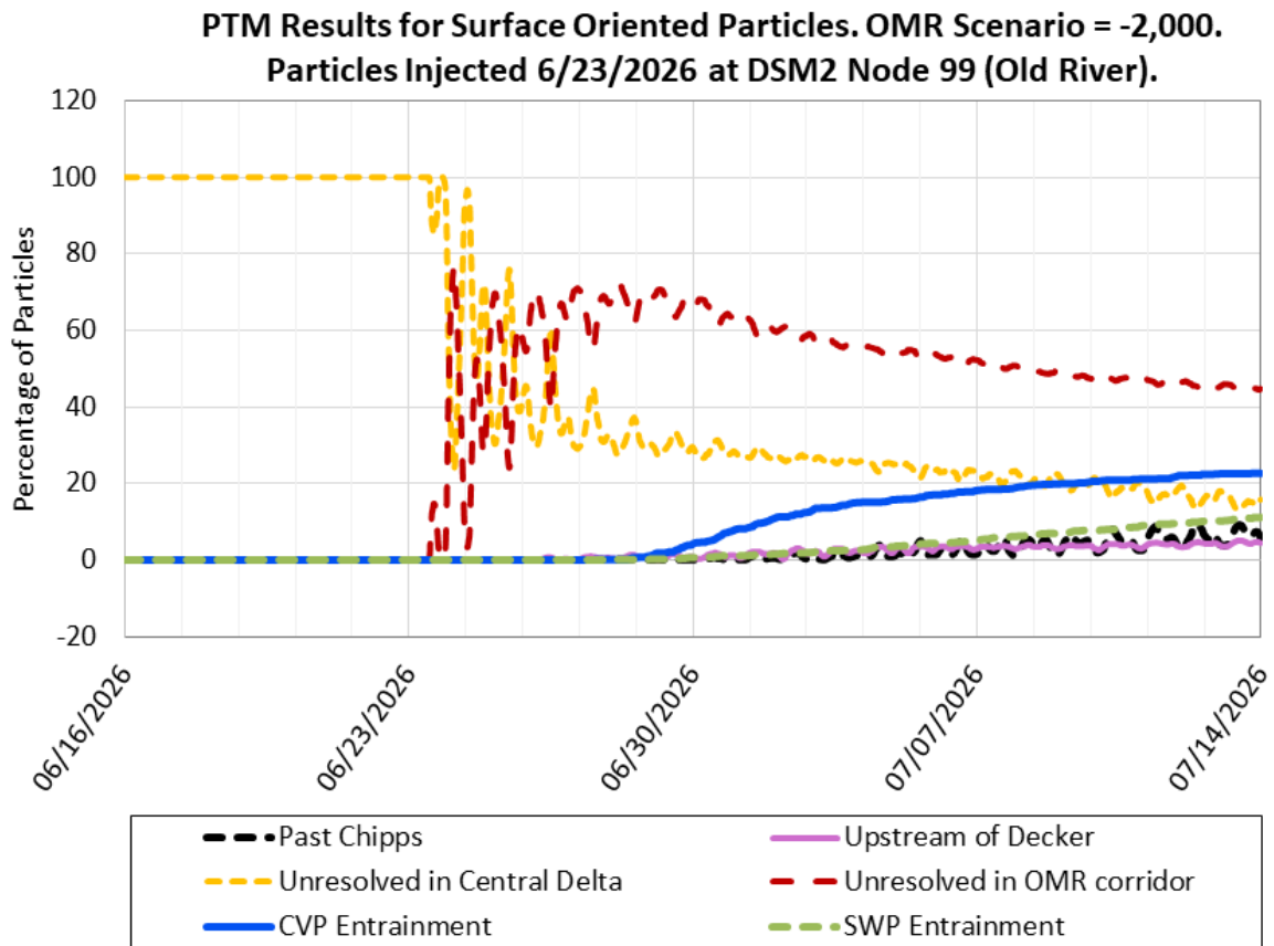
Figure 32: PTM Results for Surface Oriented Particles. OMR Scenario -2,000 cfs. Particles Injected 06/23/2026 at DSM2 Node 99 (Old River)
