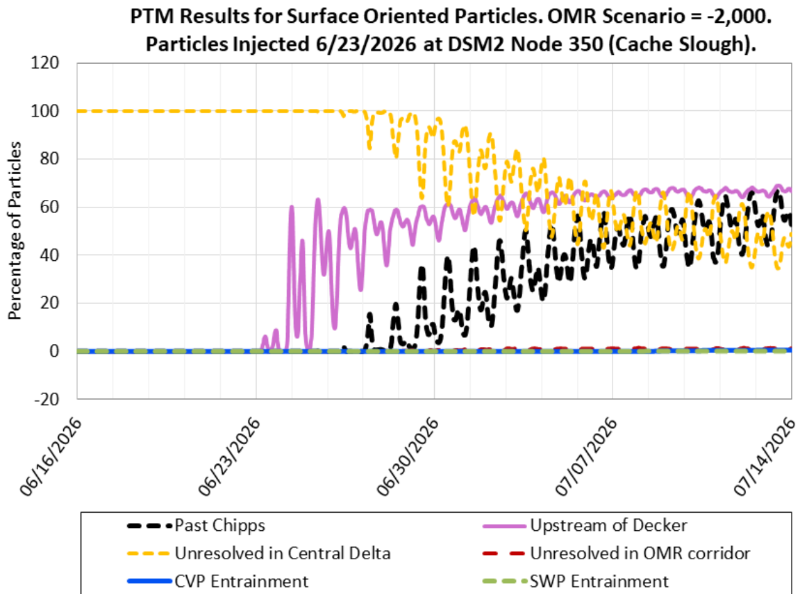
Figure 26: PTM Results for Surface Oriented Particles. OMR Scenario -2,000 cfs. Particles Injected 06/23/2026 at DSM2 Node 350 (Cache Slough)
