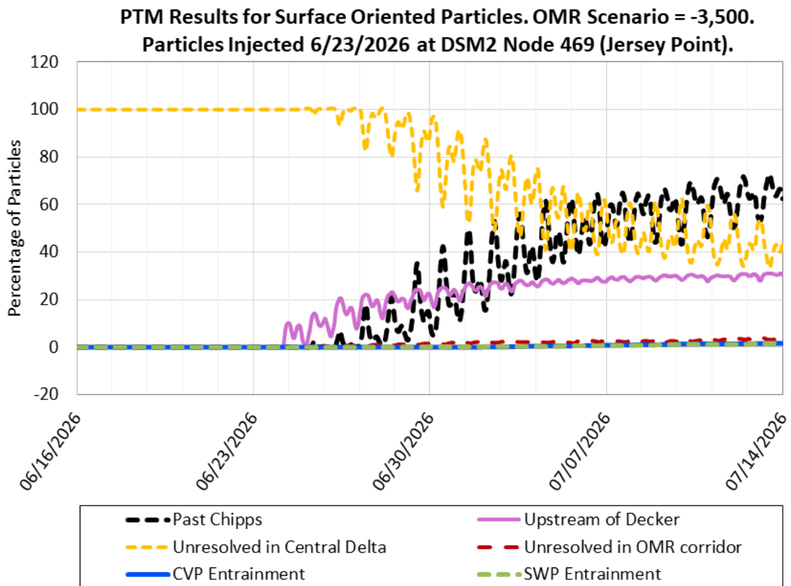
Figure 28: PTM Results for Surface Oriented Particles. OMR Scenario -3,500 cfs. Particles Injected 06/23/2026 at DSM2 Node 469 (Jersey Point)
