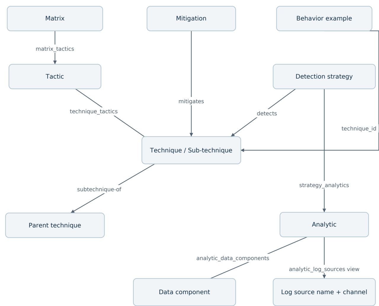
Figure 2 illustrates the core database relationships and entity connections mapped within the attack schema. For a comprehensive breakdown of the PostgreSQL schema design and table structures, please refer to Appendix A.
