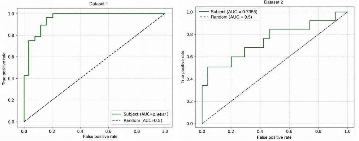
Figure S1: ROC Curve with dataset 1 and dataset 2.
