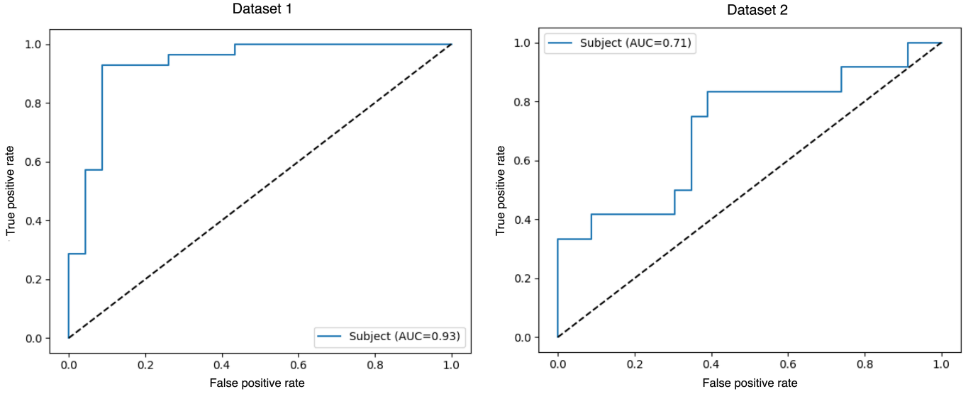
Figure S1: ROC Curve with dataset 1 and dataset 2.
