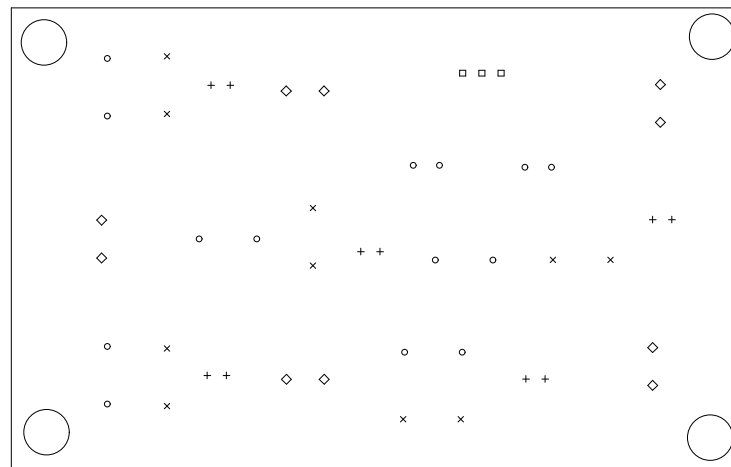
Drill Map:
