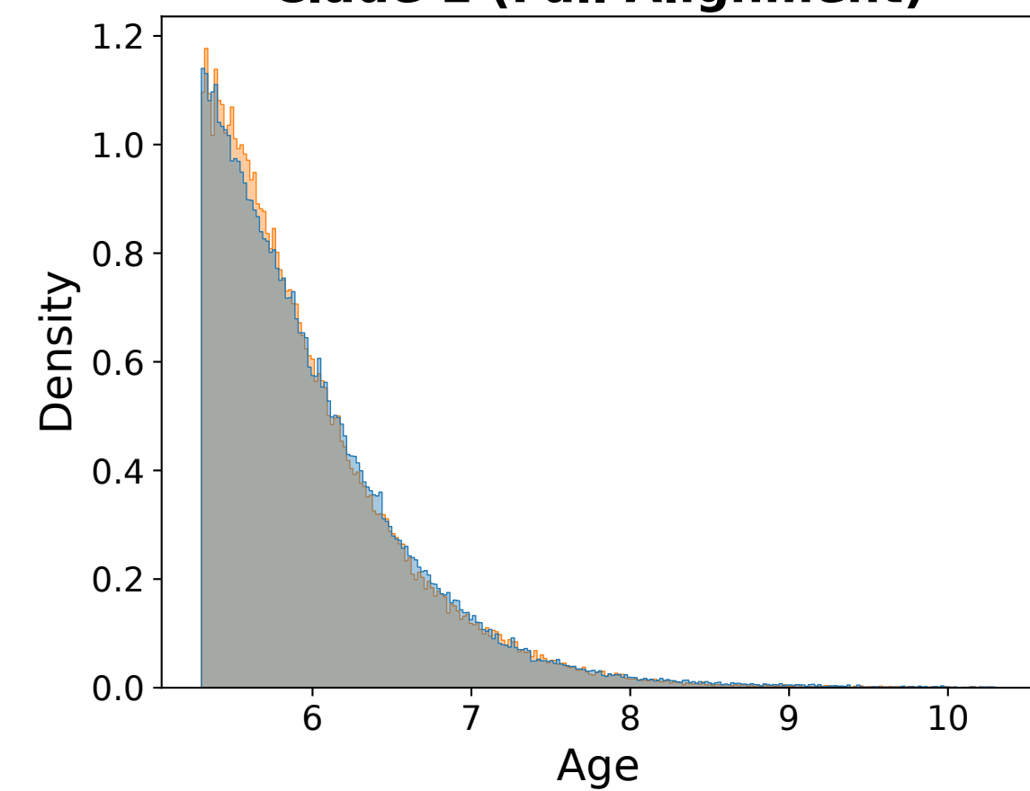
Clade 1 (Full Alignment)
