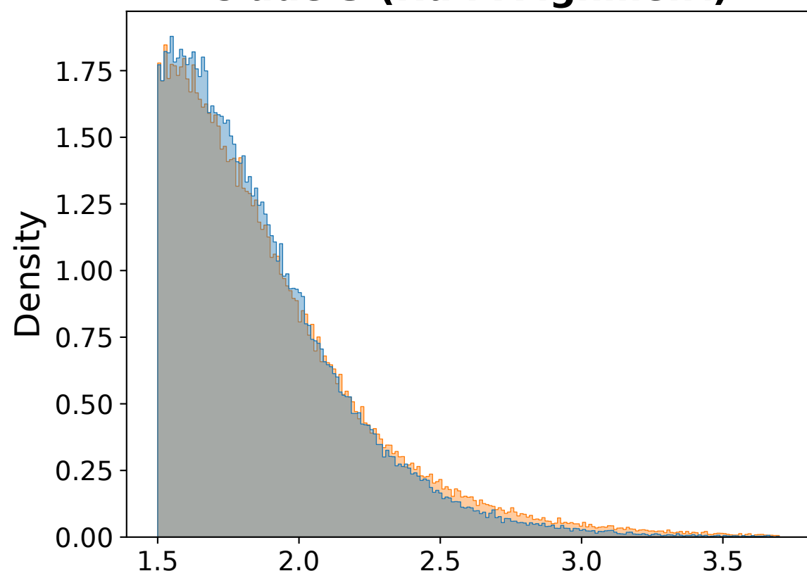
Clade 3 (Full Alignment)
