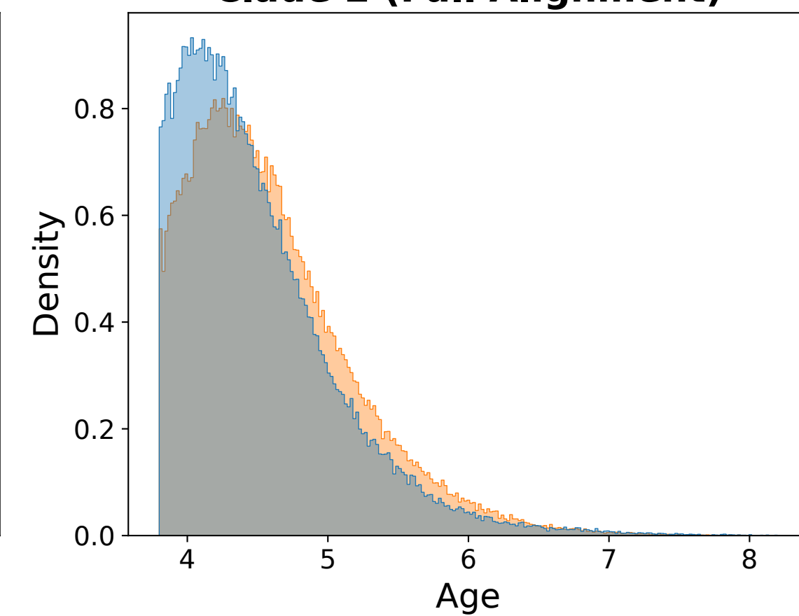
Clade 2 (Full Alignment)
