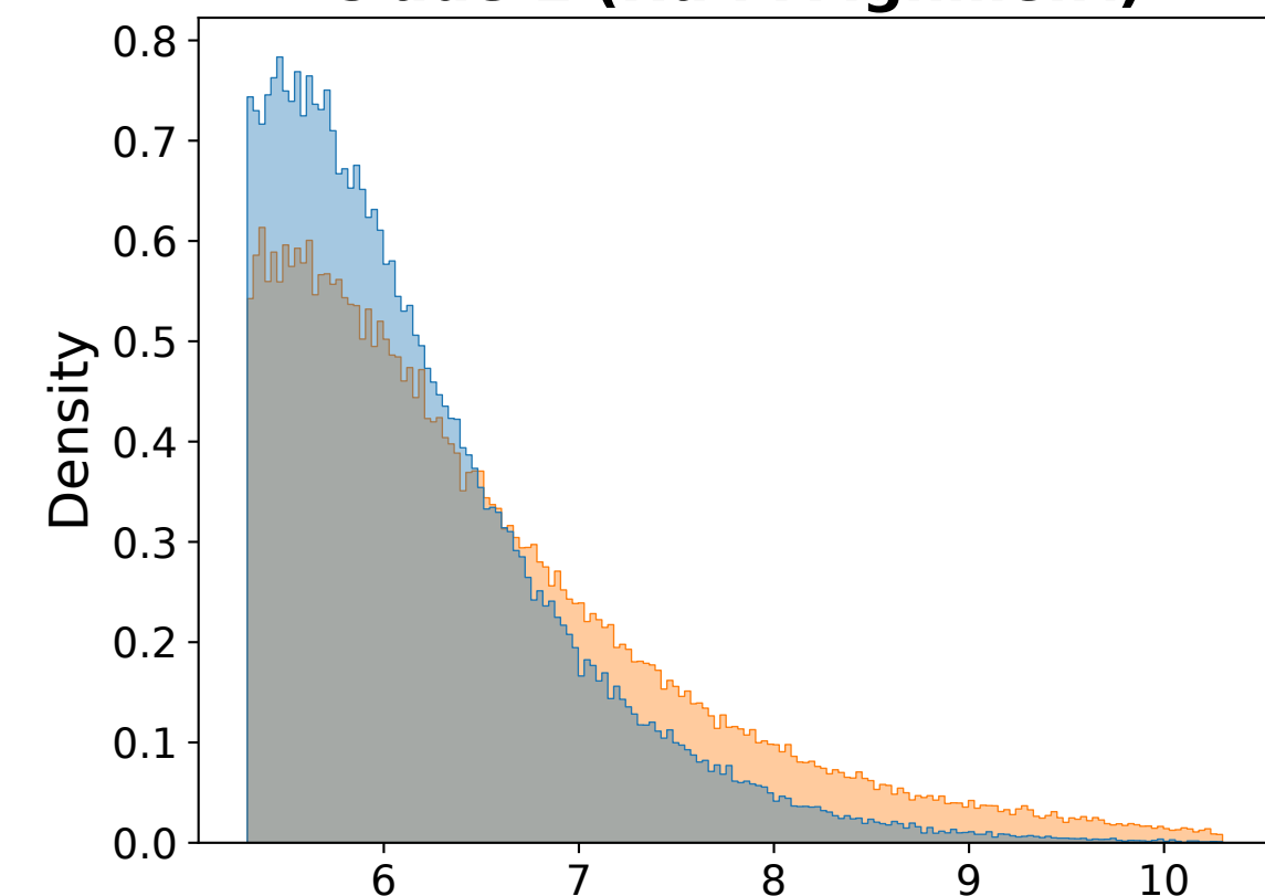
Clade 1 (Full Alignment)
