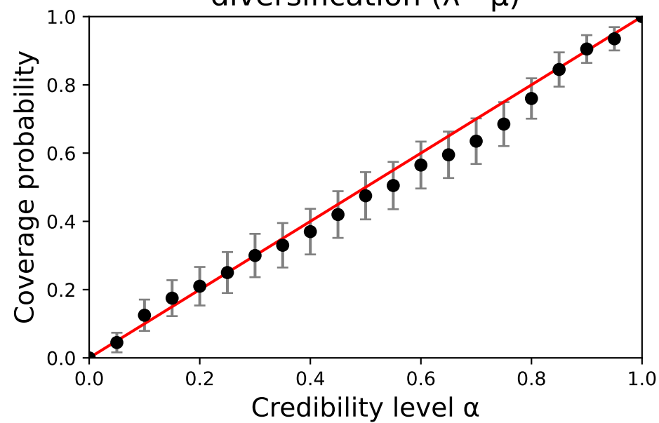
diversification ( \lambda - \mu )
