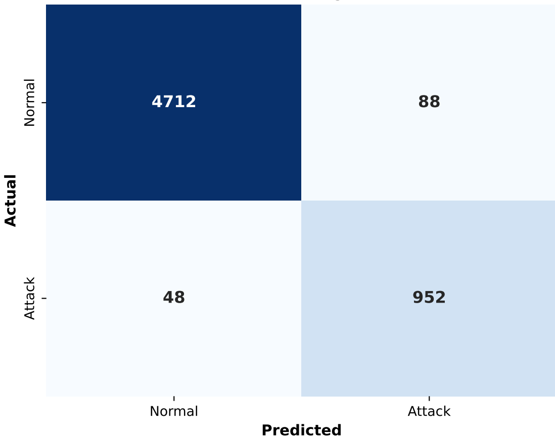
Confusion Matrix: DQN Agent Performance
