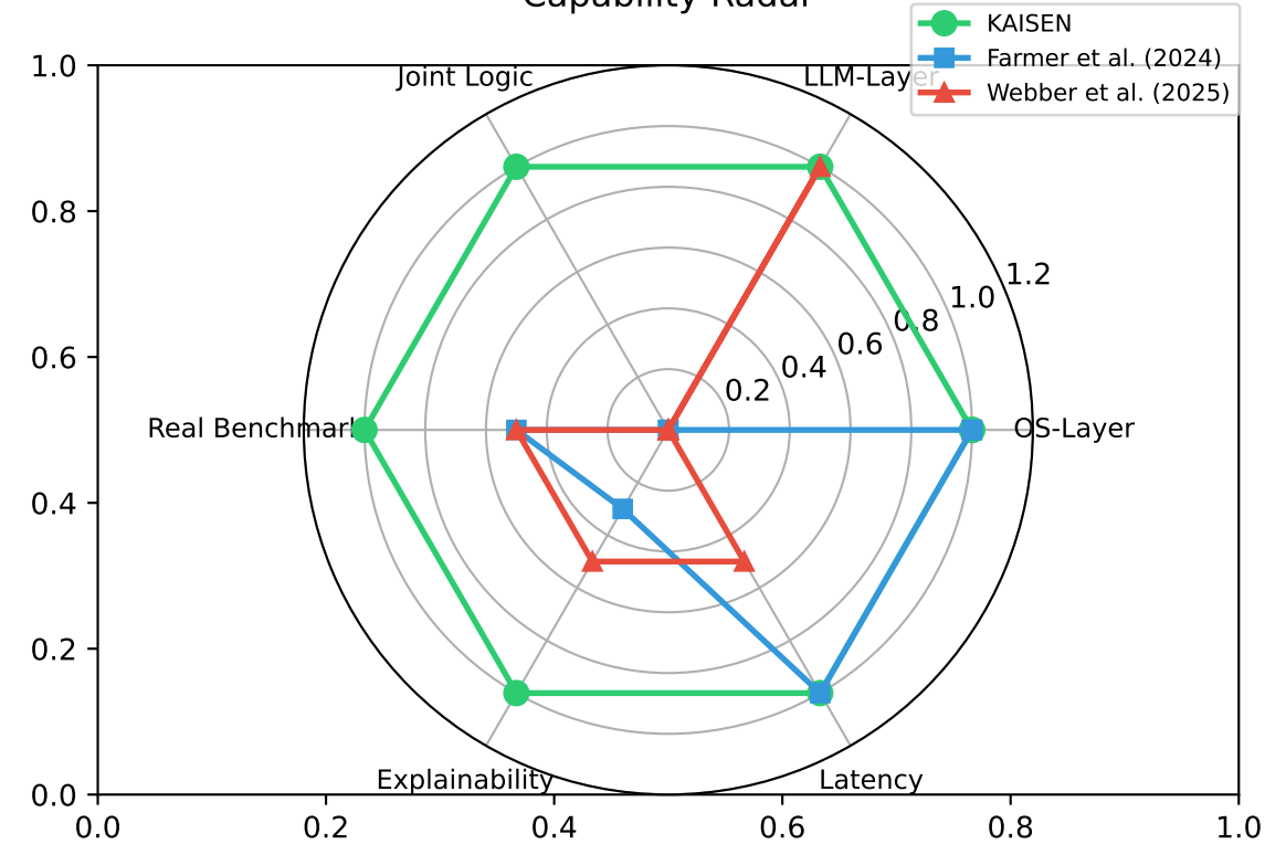
Capability Radar
