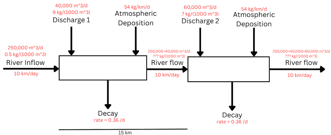
Figure 3: Systems diagram showing relevant control volumes and flows for problem 2
