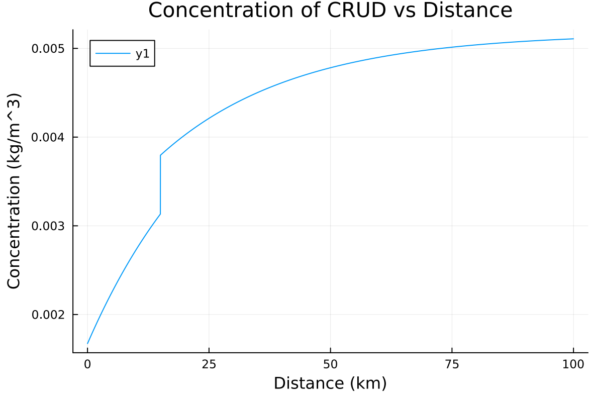
Figure 4: Numerical Forward Euler Solution plot showing concentration of CRUD vs distance for problem 2
