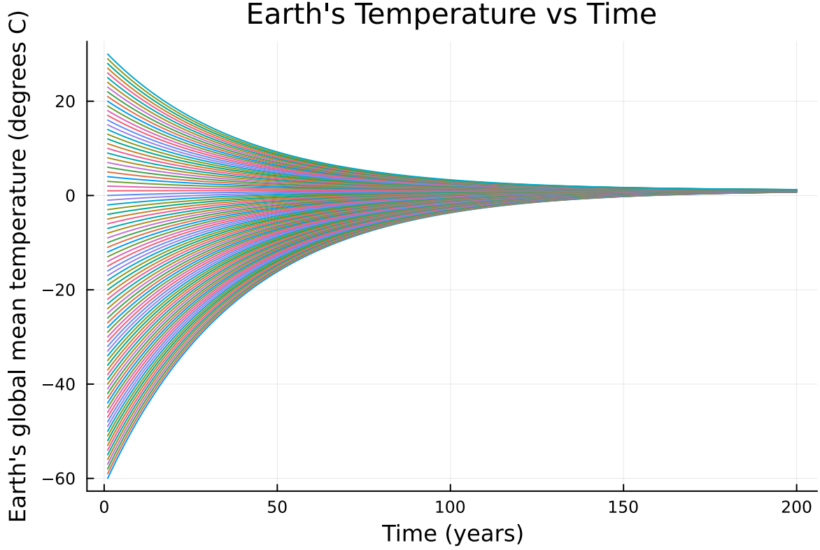
Figure 5: Earth's temperature over time using forward Euler numerical integration assuming Neoproterozoic solar constant and starting temperatures -60 to 30.
