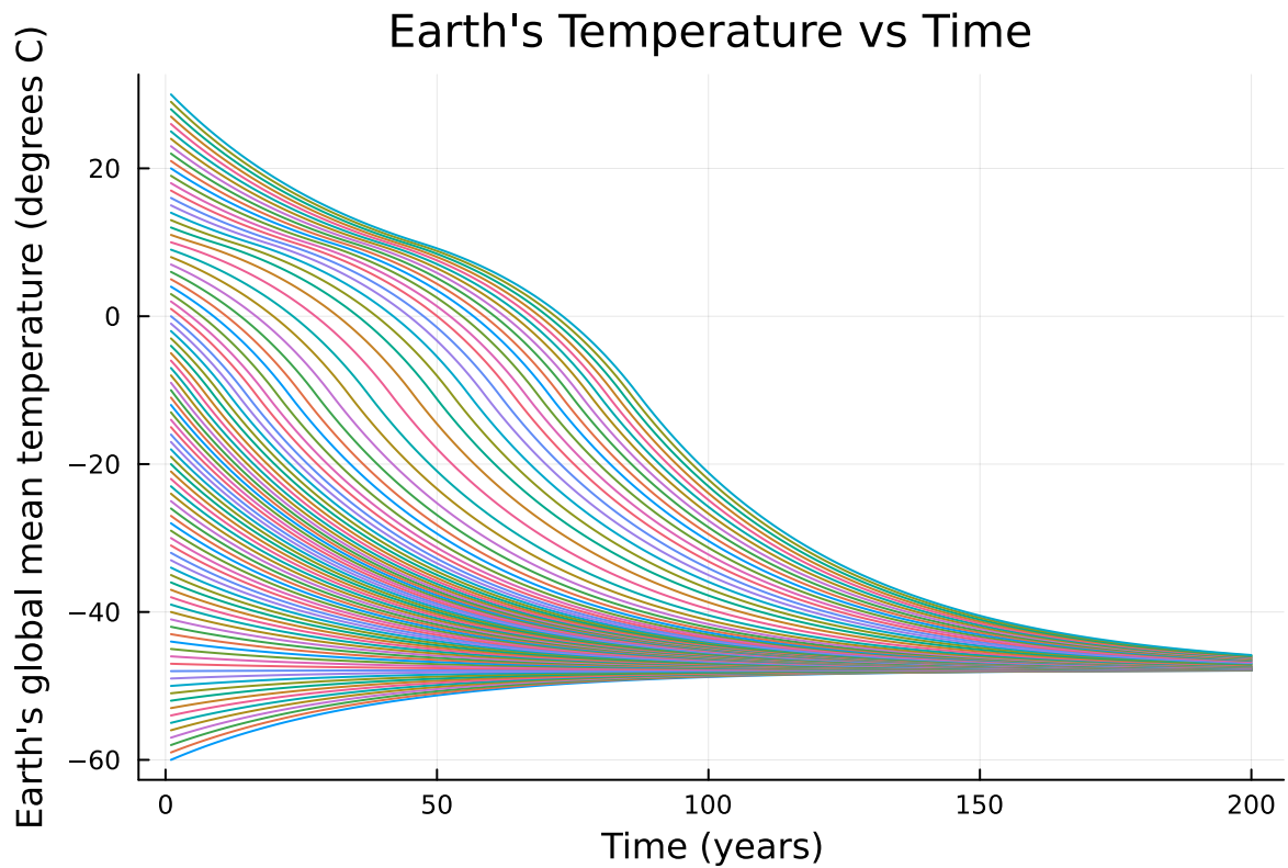
Figure 6: Earth's temperature over time using forward Euler numerical integration adjusting albedo based on temperature. Neoproterozoic solar radiation is assumed.
