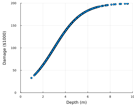
Damage vs Depth for LogNormal Distribution
