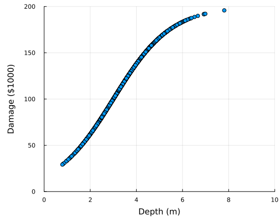
Damage vs Depth for GEV Distribution
